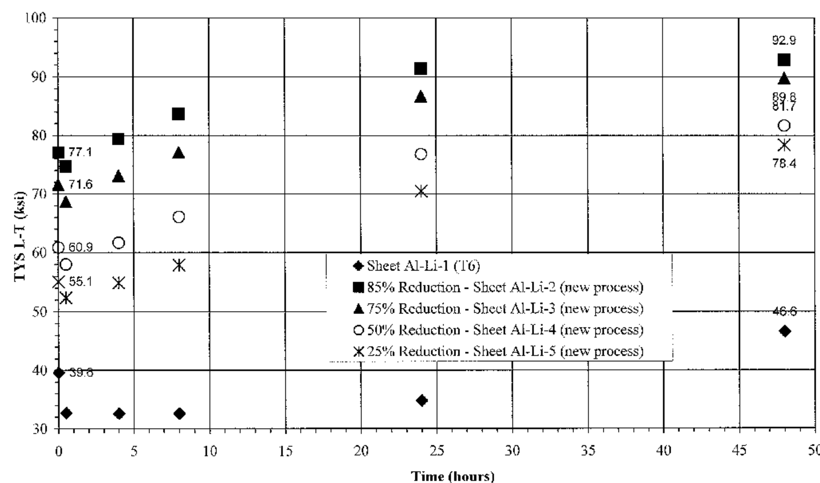
FIG. 15 - 2xxx Al-Li - TYS v. Time at 290F
