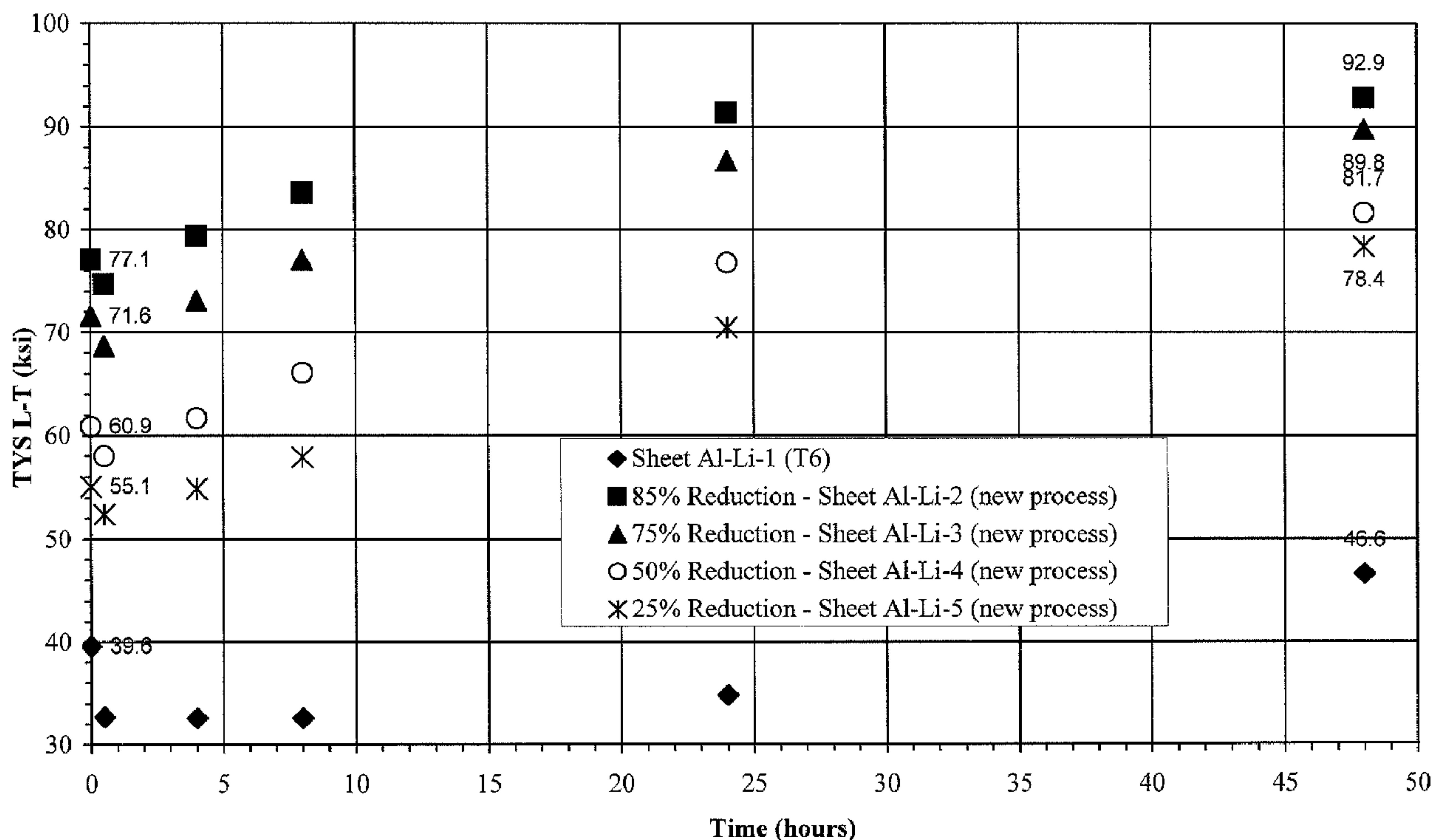
FIG. 15 - 2xxx Al-Li - TYS v. Time at 290F
