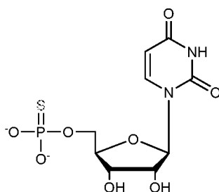
5'-O-(1-Thiophosphate)-Uridine
