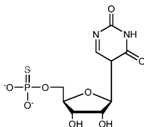
5'-O-(1-Thiophosphate)-Pseudouridine
