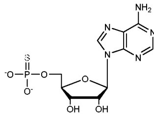
5'-O-(1-Thiophosphate)-Adenosine
