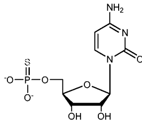
5'-O-(1-Thiophosphate)-Cytidine
