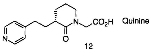
Pyridine Acid Quinine Salt MW 586
