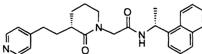
(R,R)-Diastereomer (major, RT 7.9 min)
