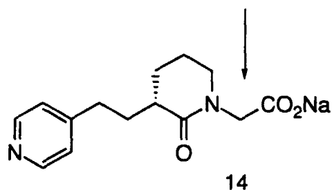
MW 262 (for free acid)
