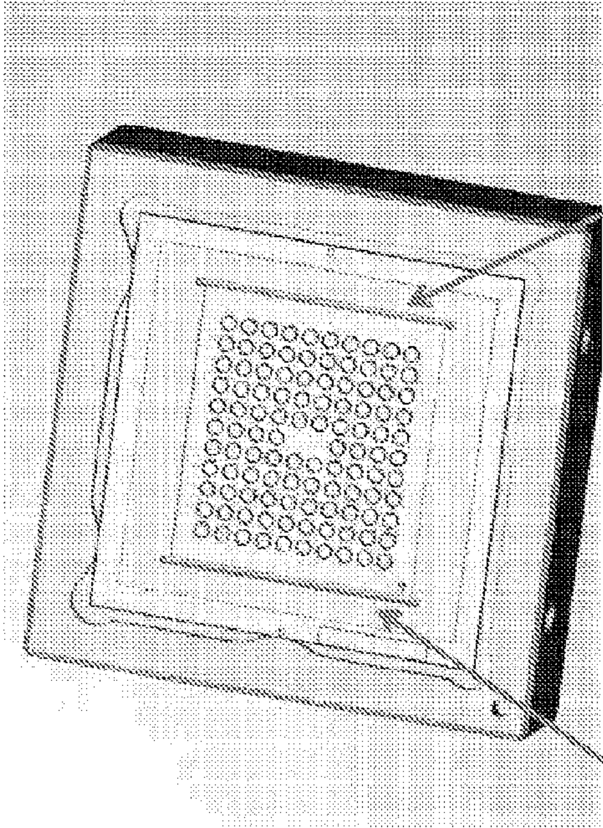
Line source Line drain Flow cell design 1 (line source, line drain)
