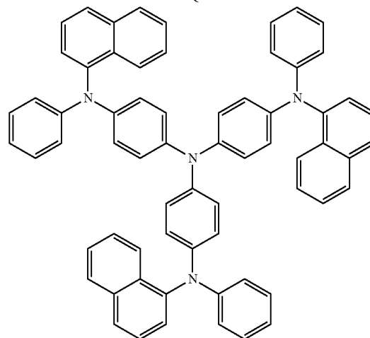
BPAPQ
