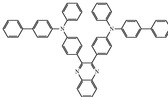
BPAPQ
