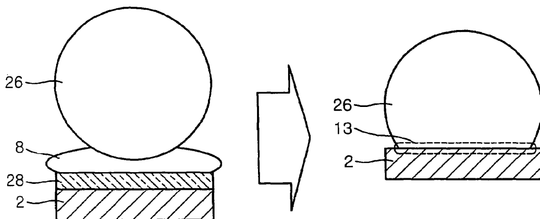
FIG. 5 (CONVENTIONAL ART)
