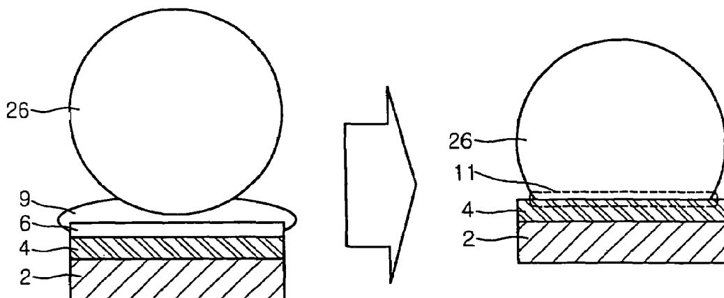
FIG. 3 (CONVENTIONAL ART)
