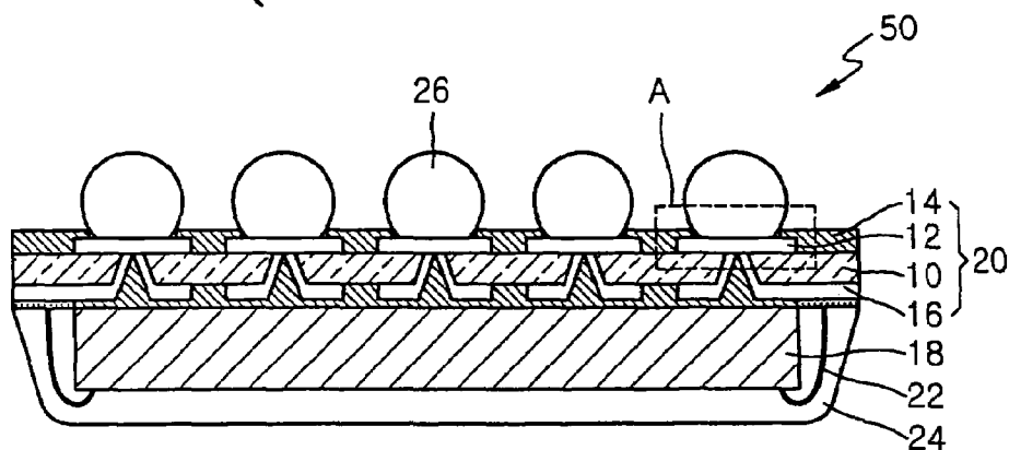
FIG. 1 (CONVENTIONAL ART)
