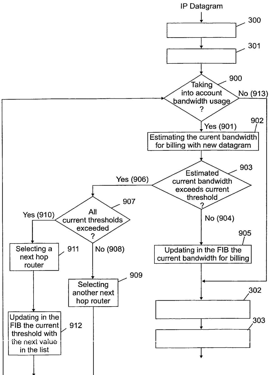
FIG. 9: Link Selection Algorithm
