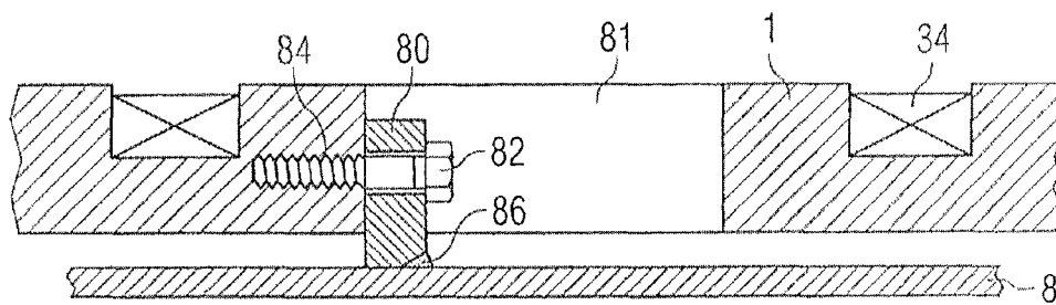
PRIOR ART
