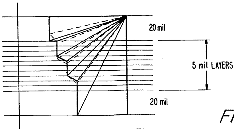
VARIABLE LAYER THICKNESS OF 5 mil AND 20 mil
