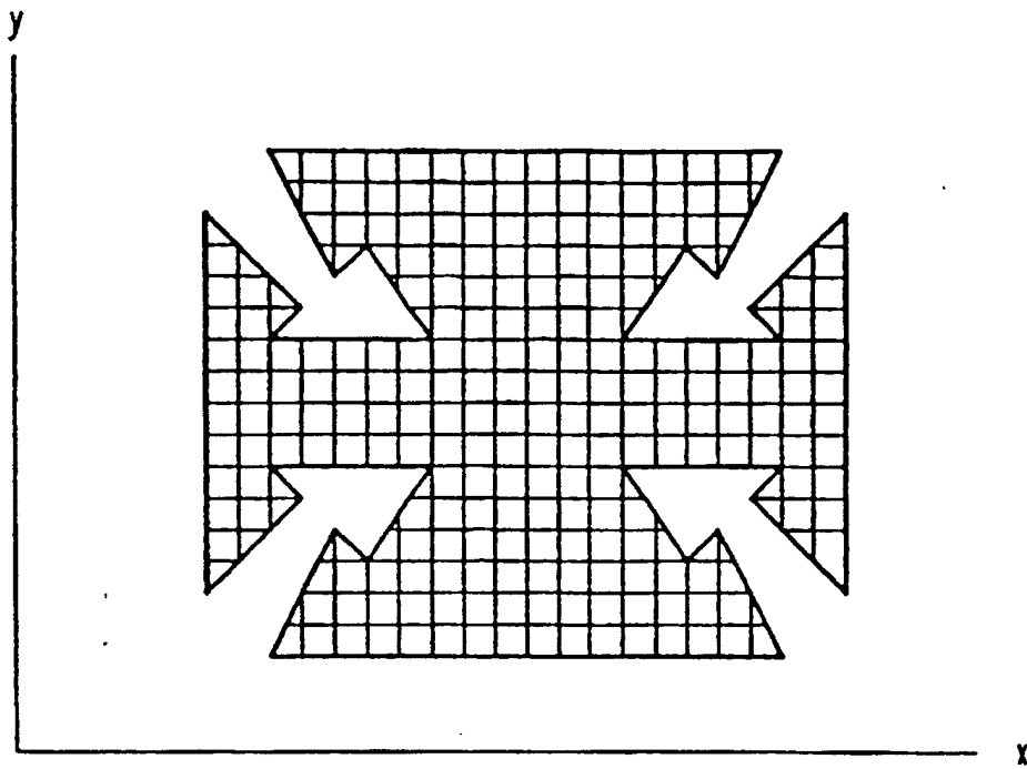
A TOP VIEW OF A LAYER OF BOUNDARY VECTORS ALONG WITH HATCH VECTORS GENERATED BY THE PROPOSED ALGORITHM ( x AND y )
