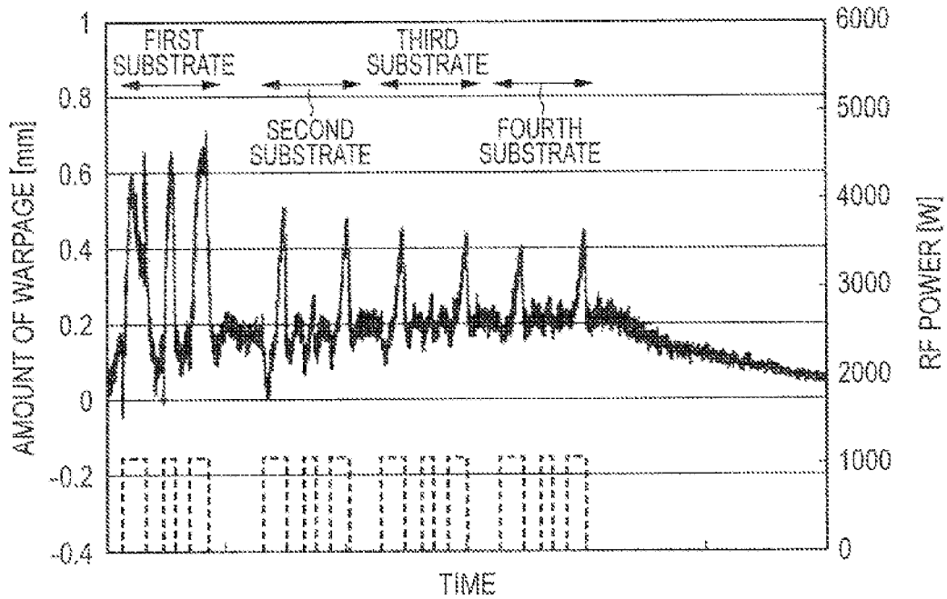
FIG. 9C PRIOR ART
