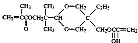
Compound 9 55
