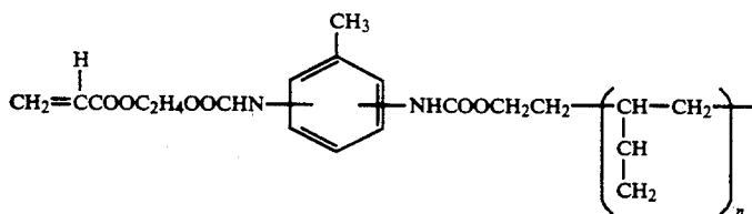
Compound 3
