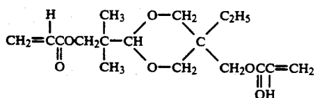
Compound 8 50
