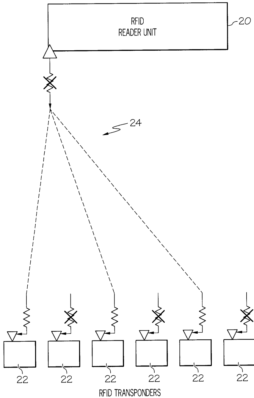
FIG. 3 (PRIOR ART)
