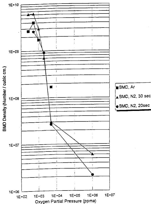
BMD Density vs. Oxygen Partial Pressure
