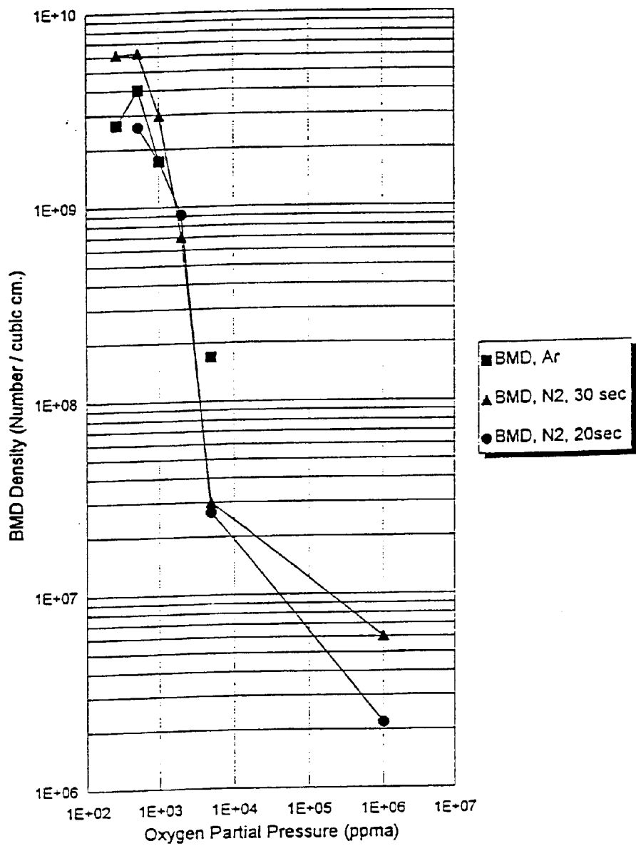
BMD Density vs. Oxygen Partial Pressure
