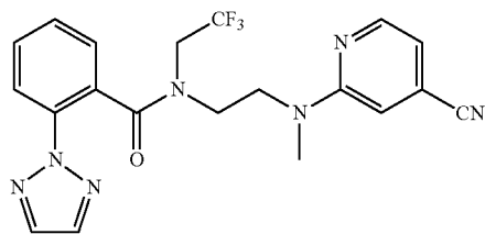
N-(2-((4-cyanopyridin-2-yl)(methyl)amino)ethyl)-2-(2H-1,2,3-triazol-2-yl)-N-(2,2,2-trifluoroethyl)benzamide (Example G-10)
