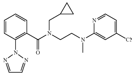
N-(2-((4-cyanopyridin-2-yl)(methyl)amino)ethyl)-N-(cyclopropylmethyl)-2-(2H-1,2,3-triazol-2-yl)benzamide (Example G-7)
