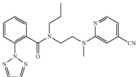
N-(2-((4-cyanopyridin-2-yl)(methyl)amino)ethyl)-N-propyl-2-(2H-1,2,3-triazol-2-yl)benzamide (Example G-4)
