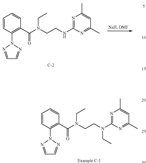
N-(2-((4,6-dimethylpyrimidin-2-yl)(ethyl)amino)ethyl)-N-ethyl-2-(2H-1,2,3-triazol-2-yl)benzamide (Example C-1)
