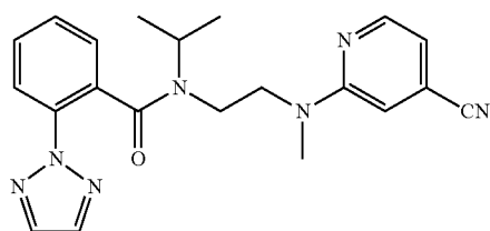
N-(2-((4-cyanopyridin-2-yl)(methyl)amino)ethyl)-N-isopropyl-2-(2H-1,2,3-triazol-2-yl)benzamide (Example G-9)
