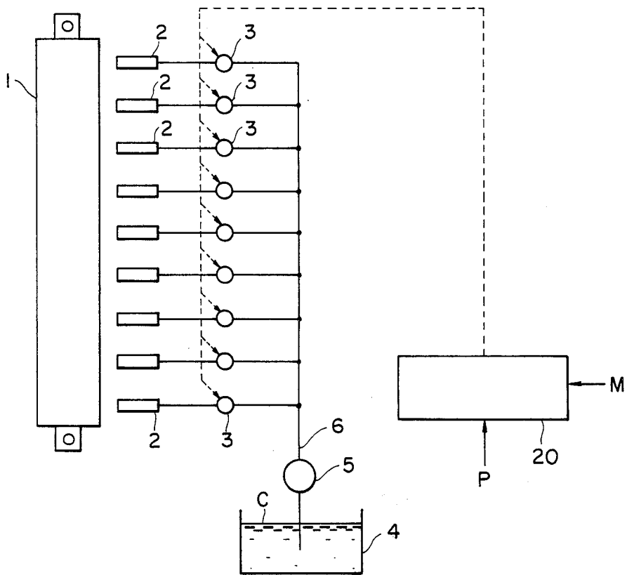
FIGURE 1 PRIOR ART
