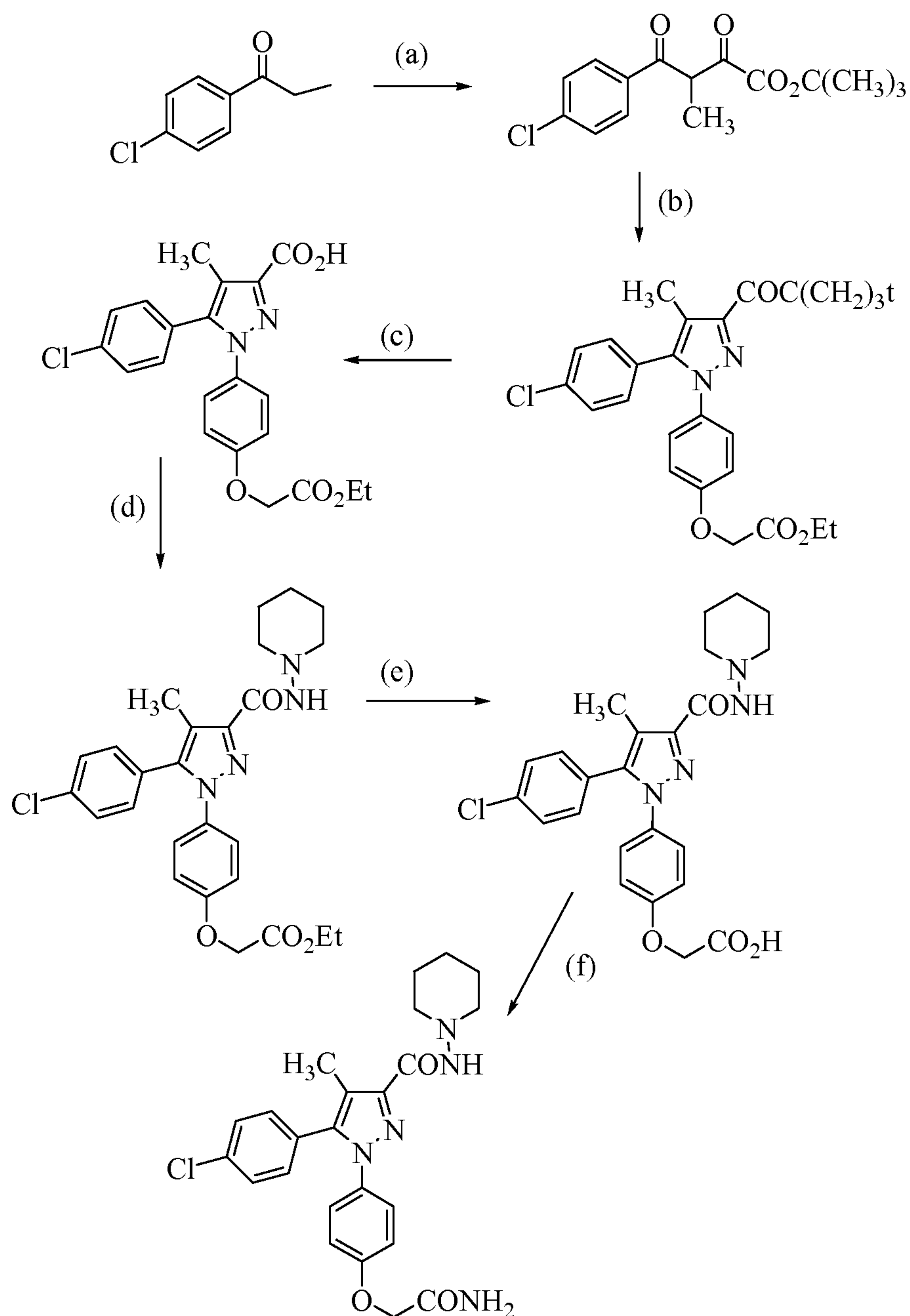
[00174] Scheme 9
