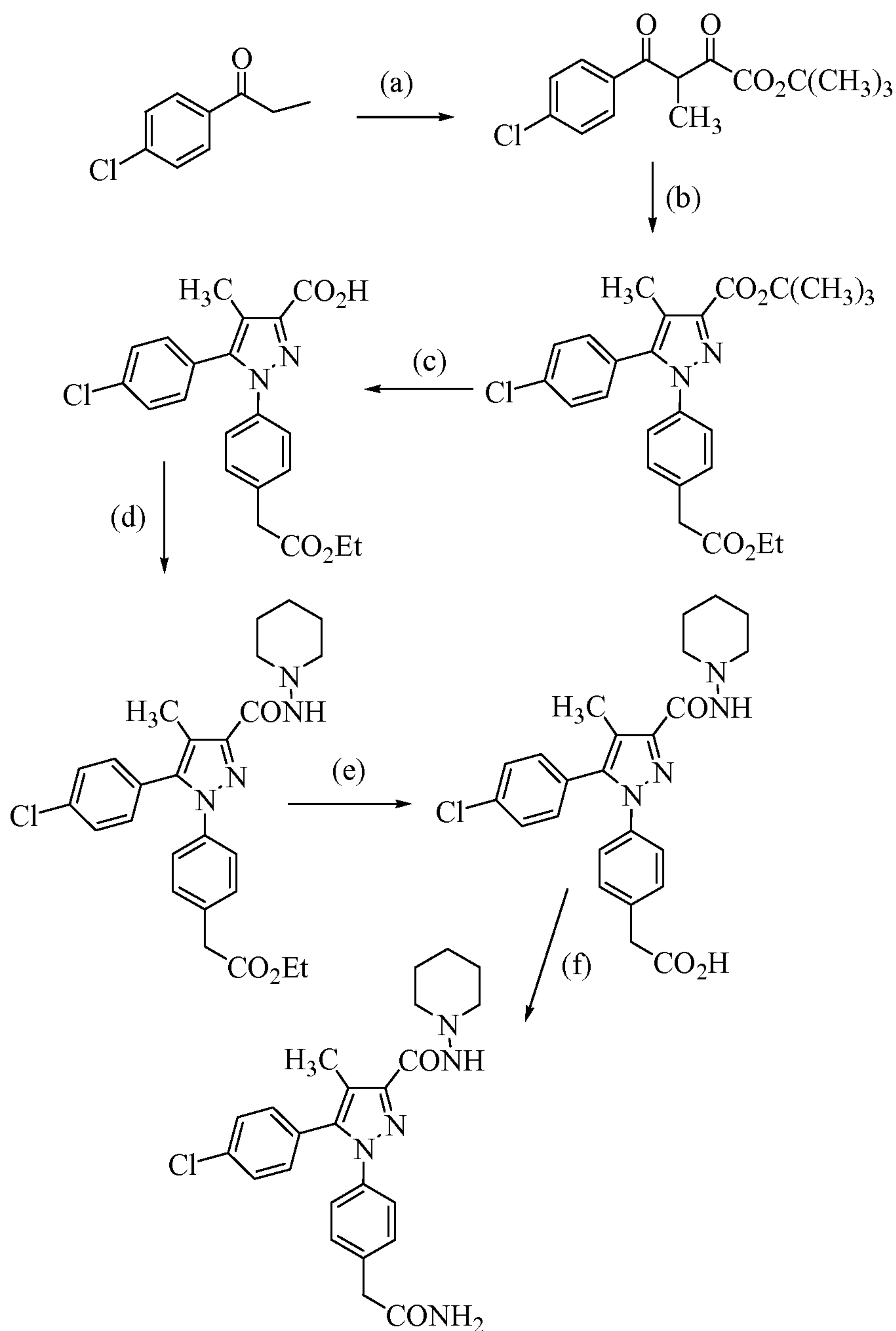
[00170] Scheme 7
