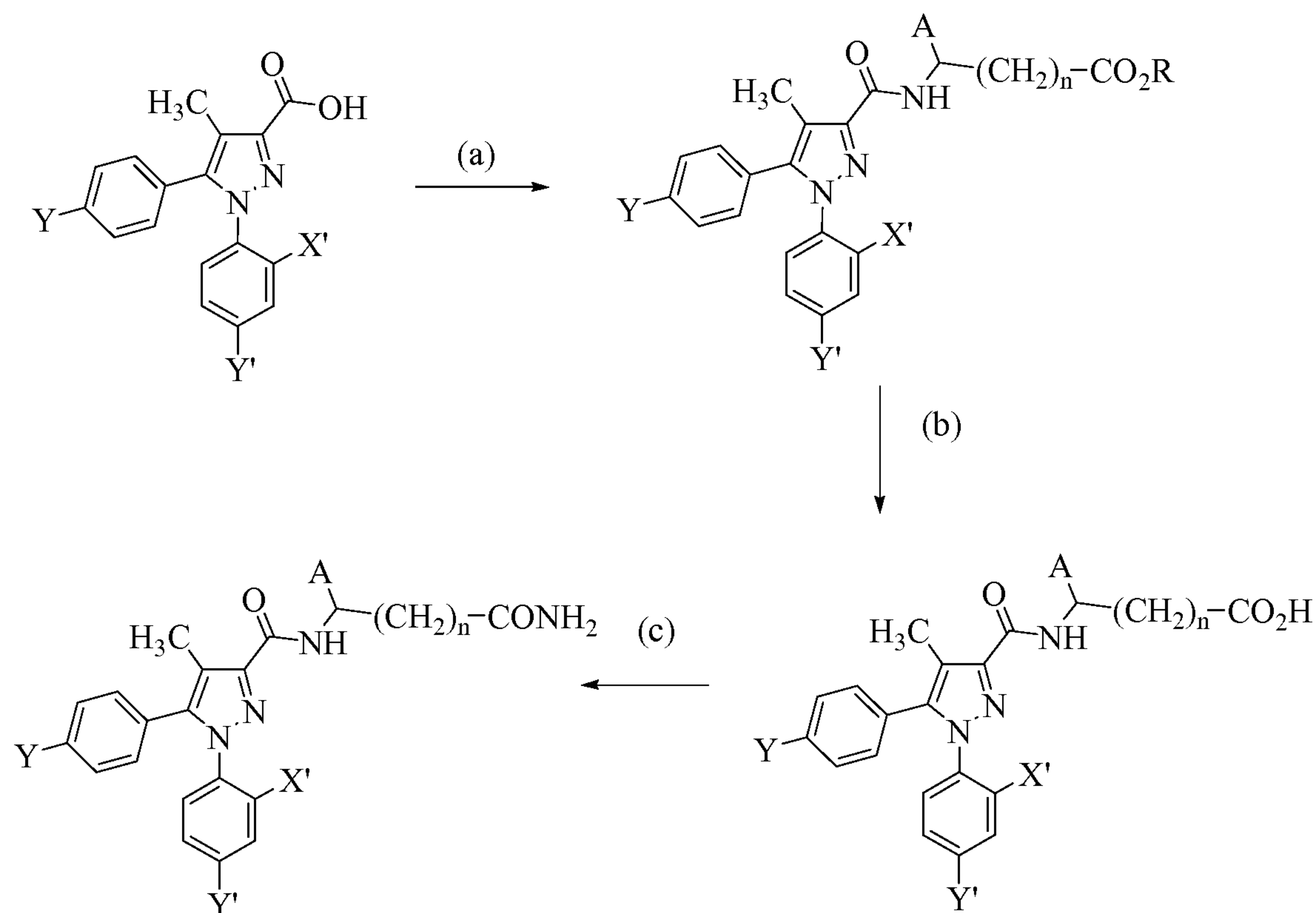
[00161] Scheme 3
