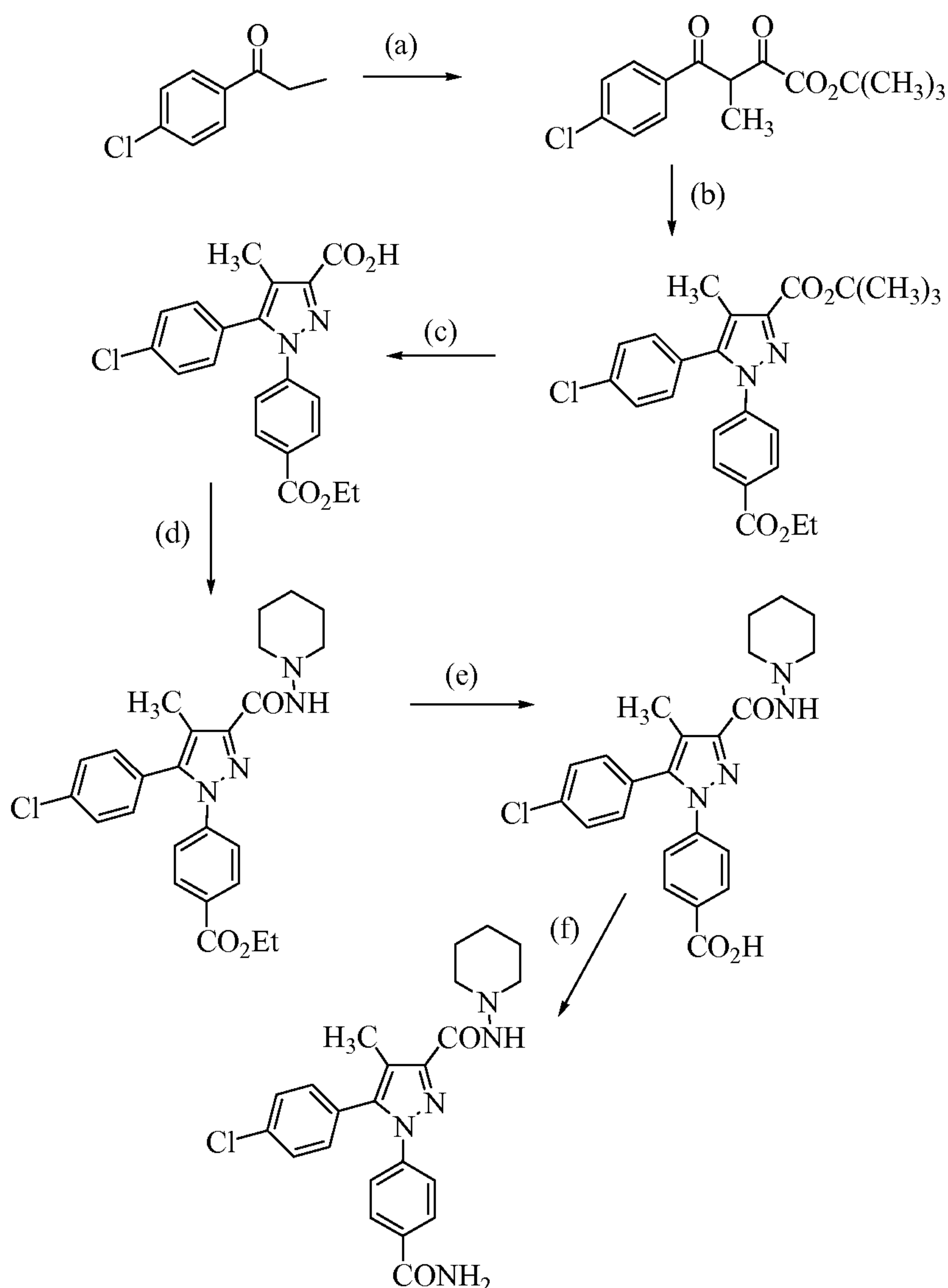
[00172] Scheme 8
