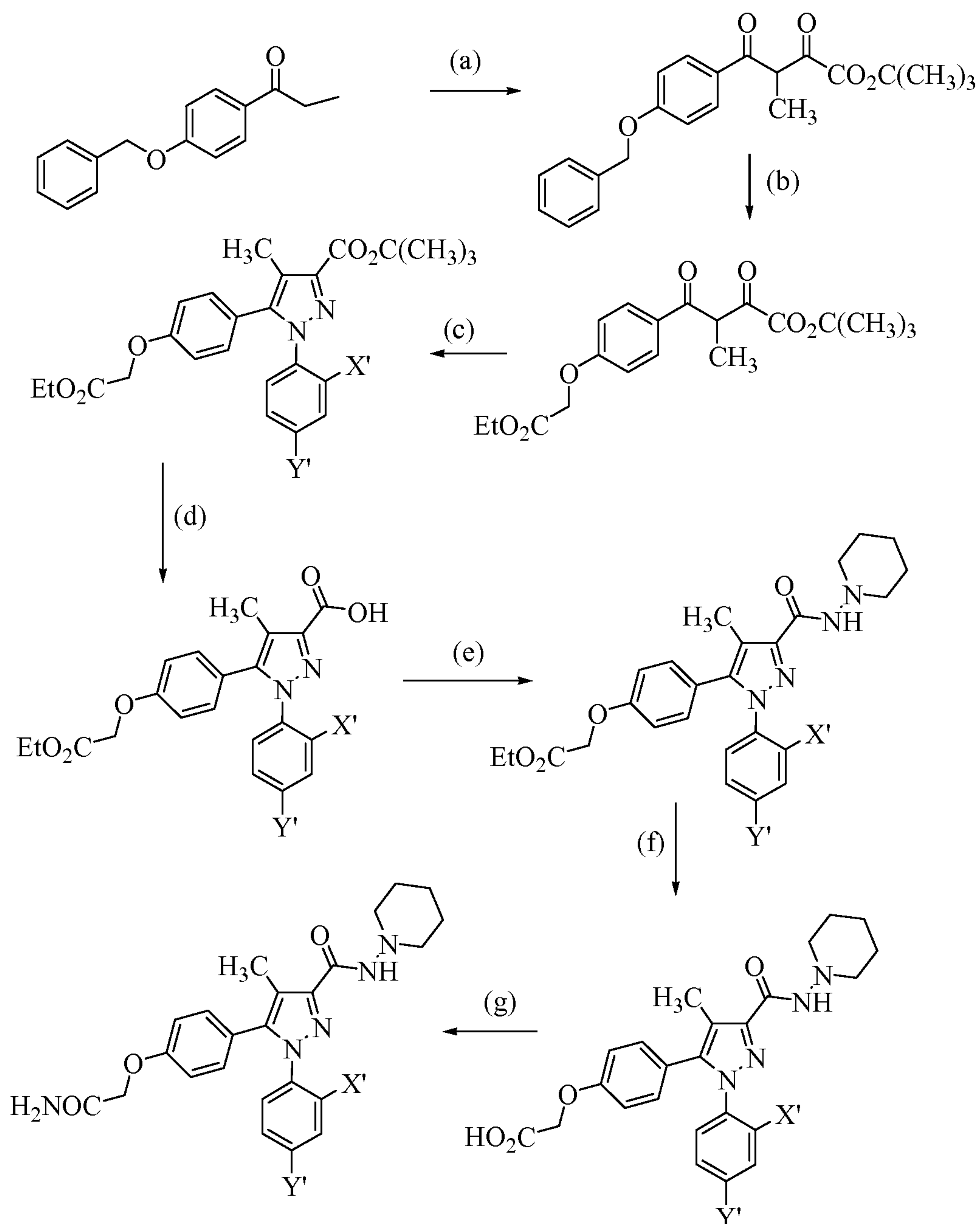
[00163] Scheme 4
