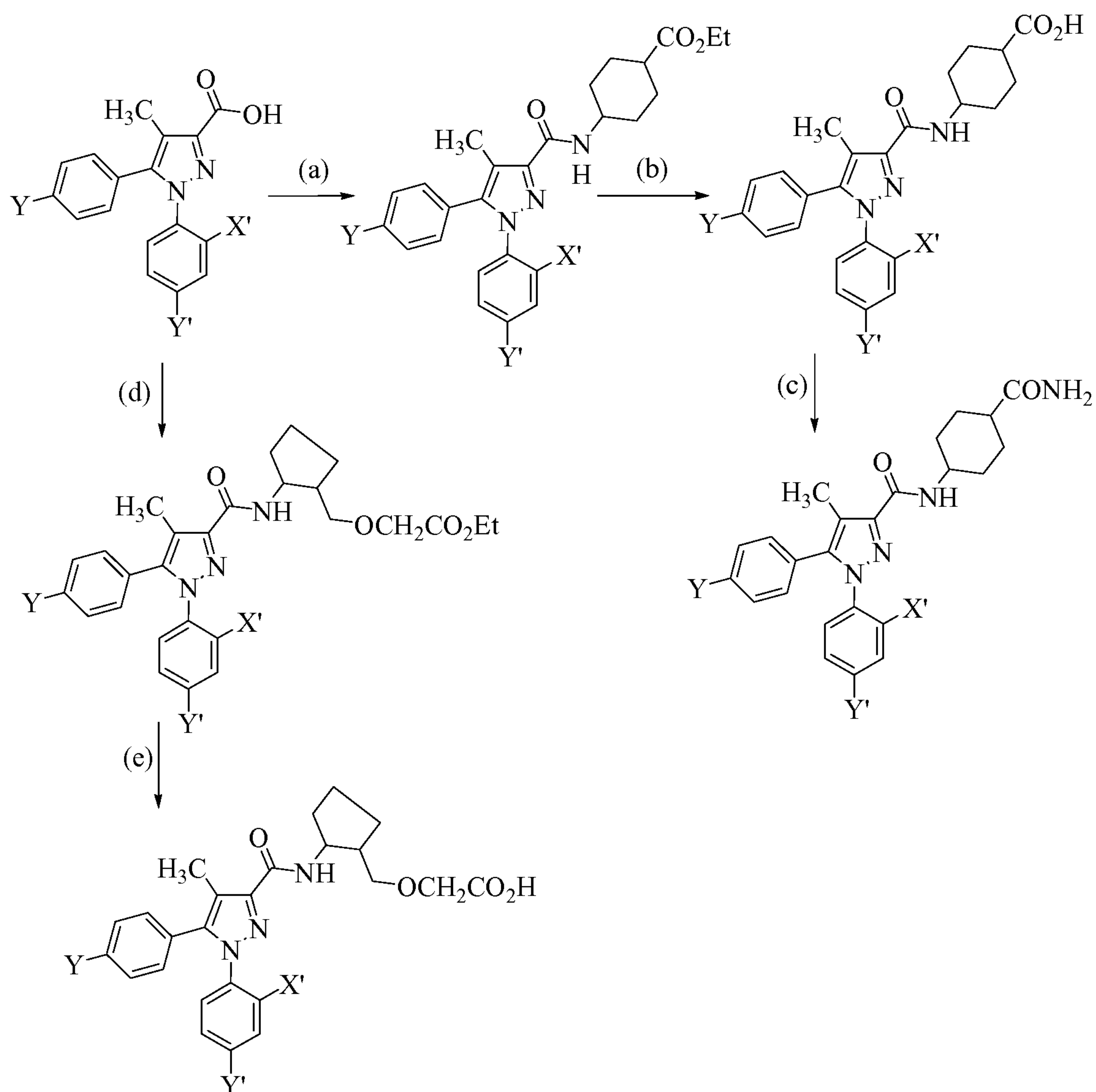
[00158] Scheme 2
