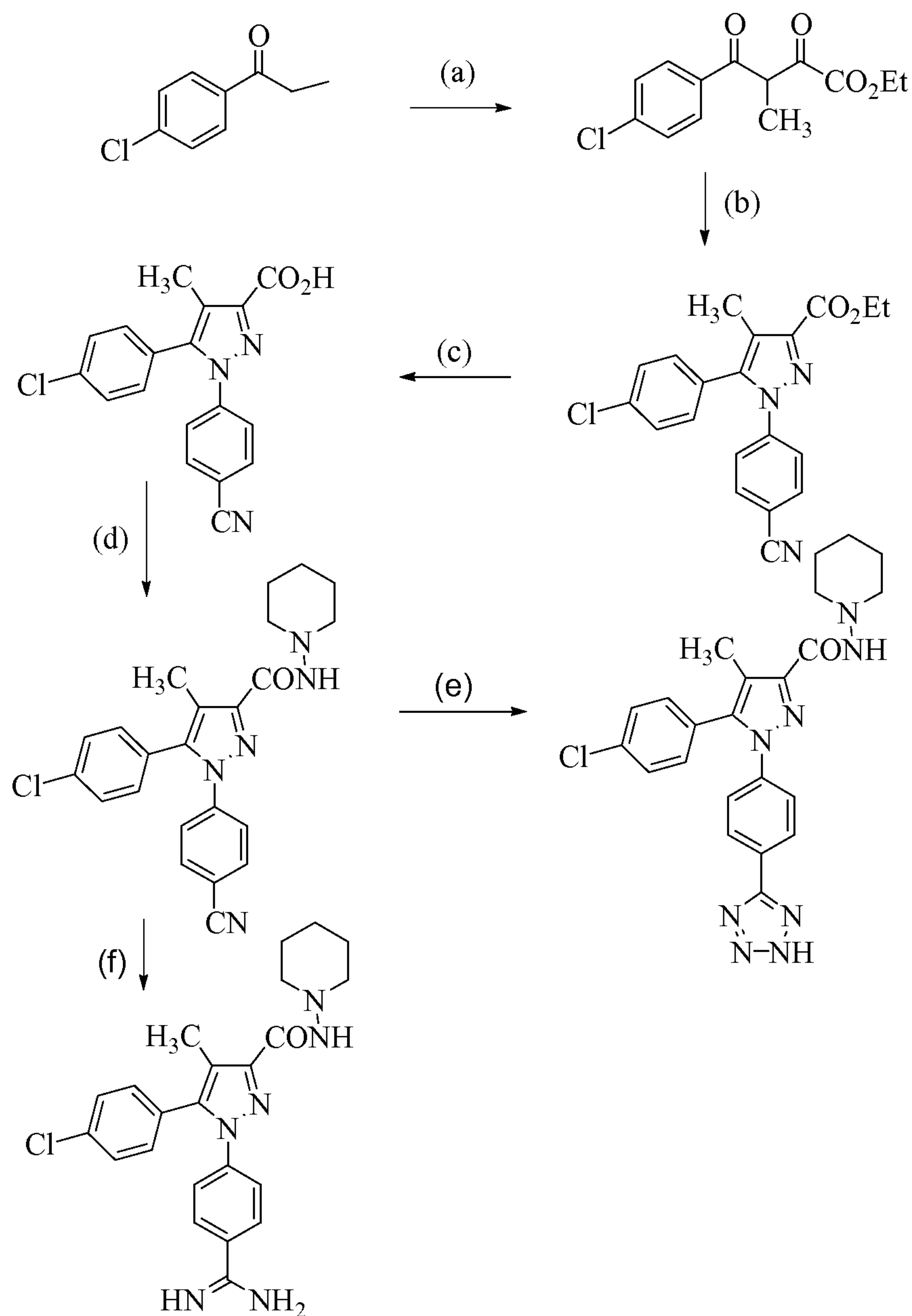
[00176] Scheme 10
