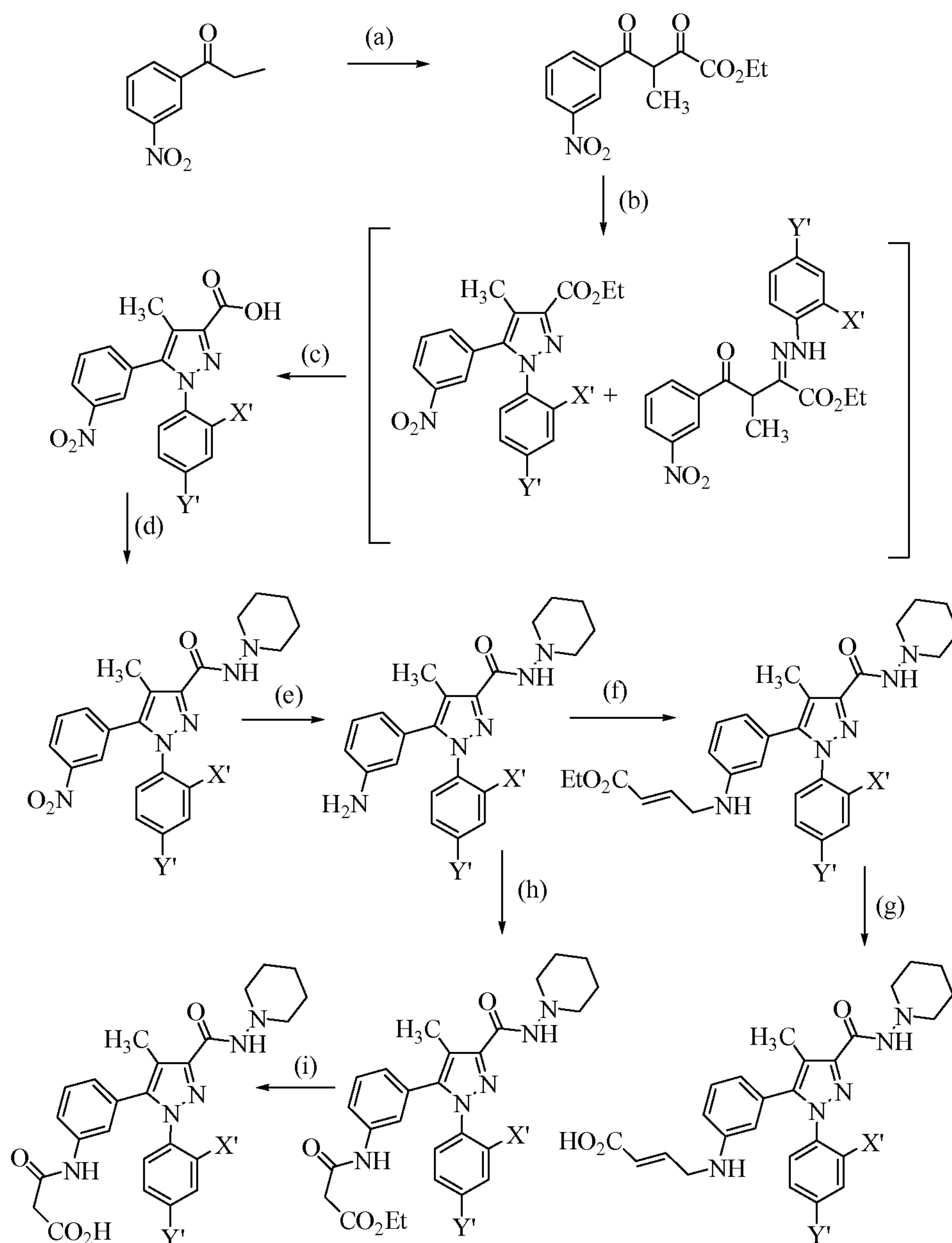
[00165] Scheme 5
