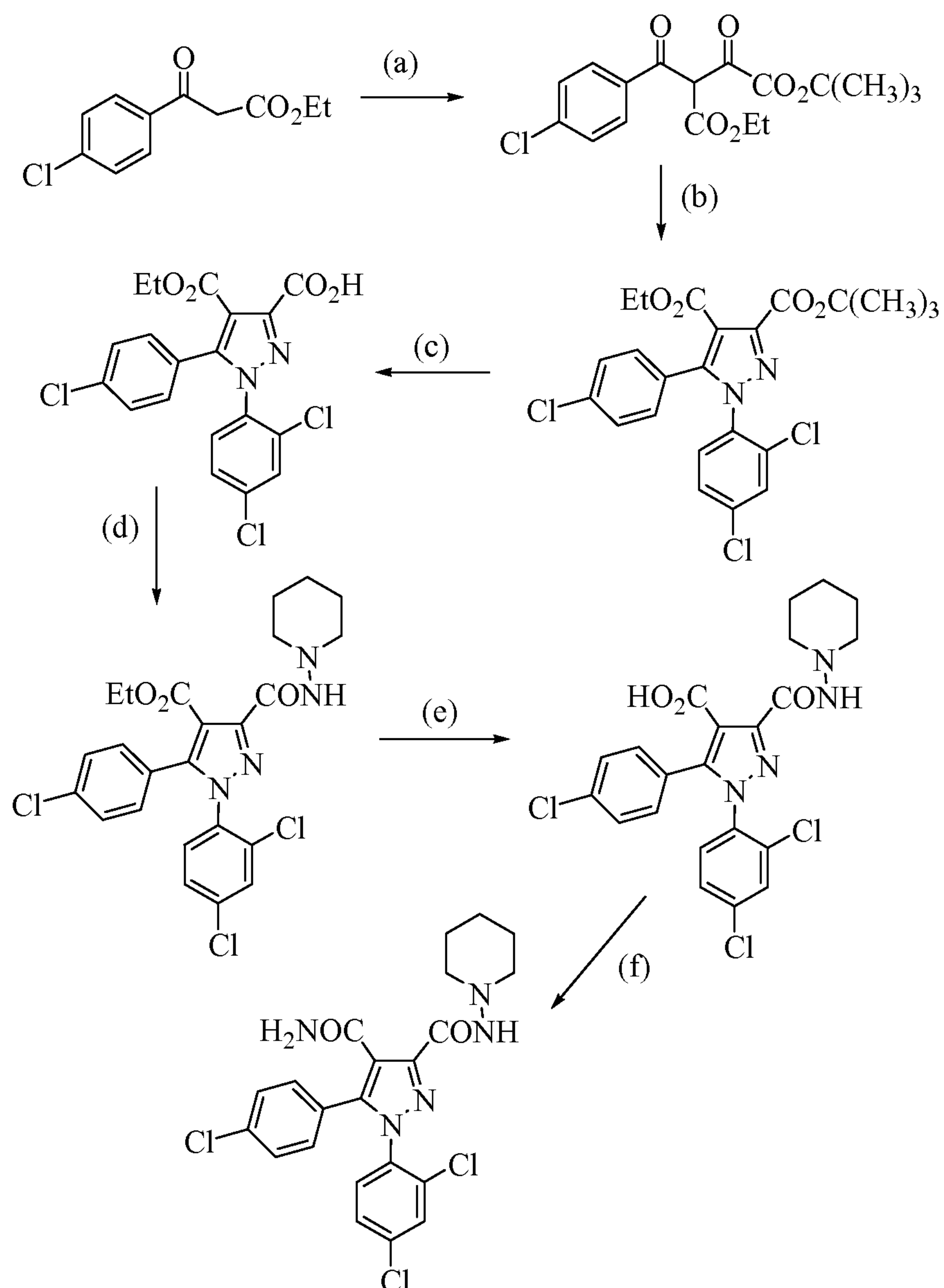
[00178] Scheme 11
