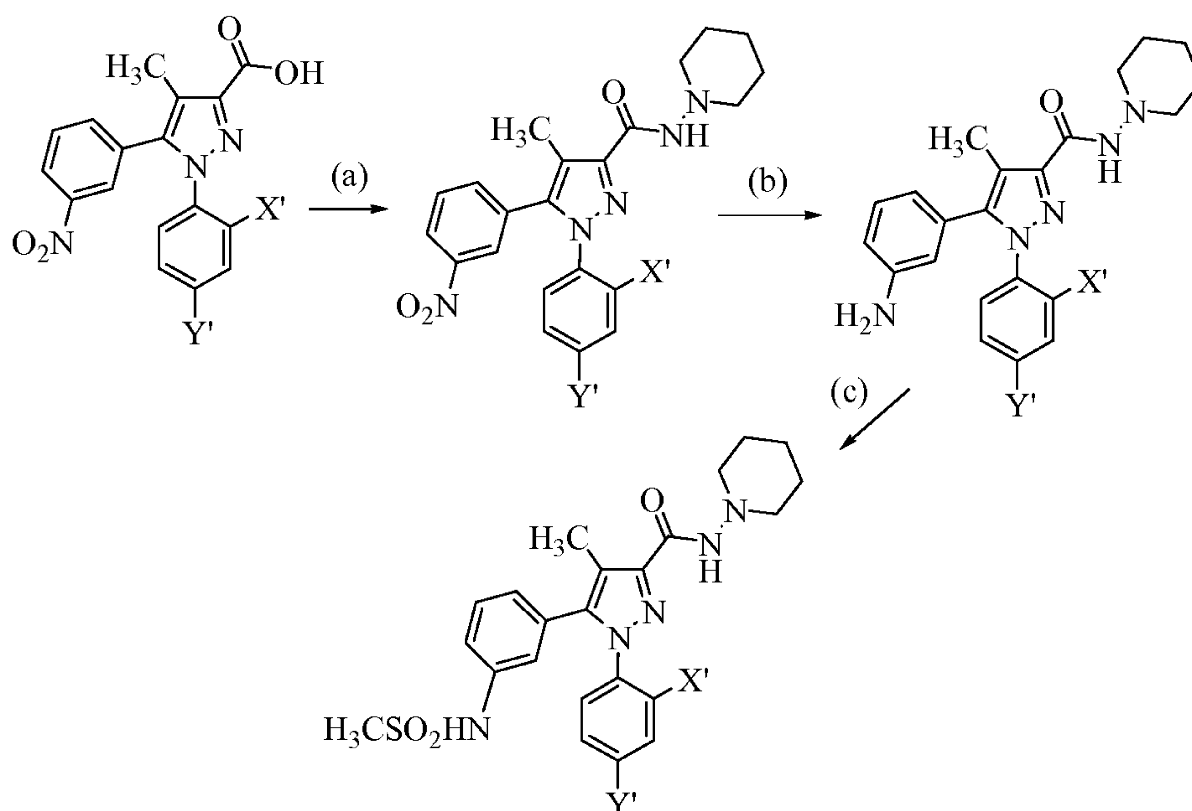
[00168] Scheme 6
