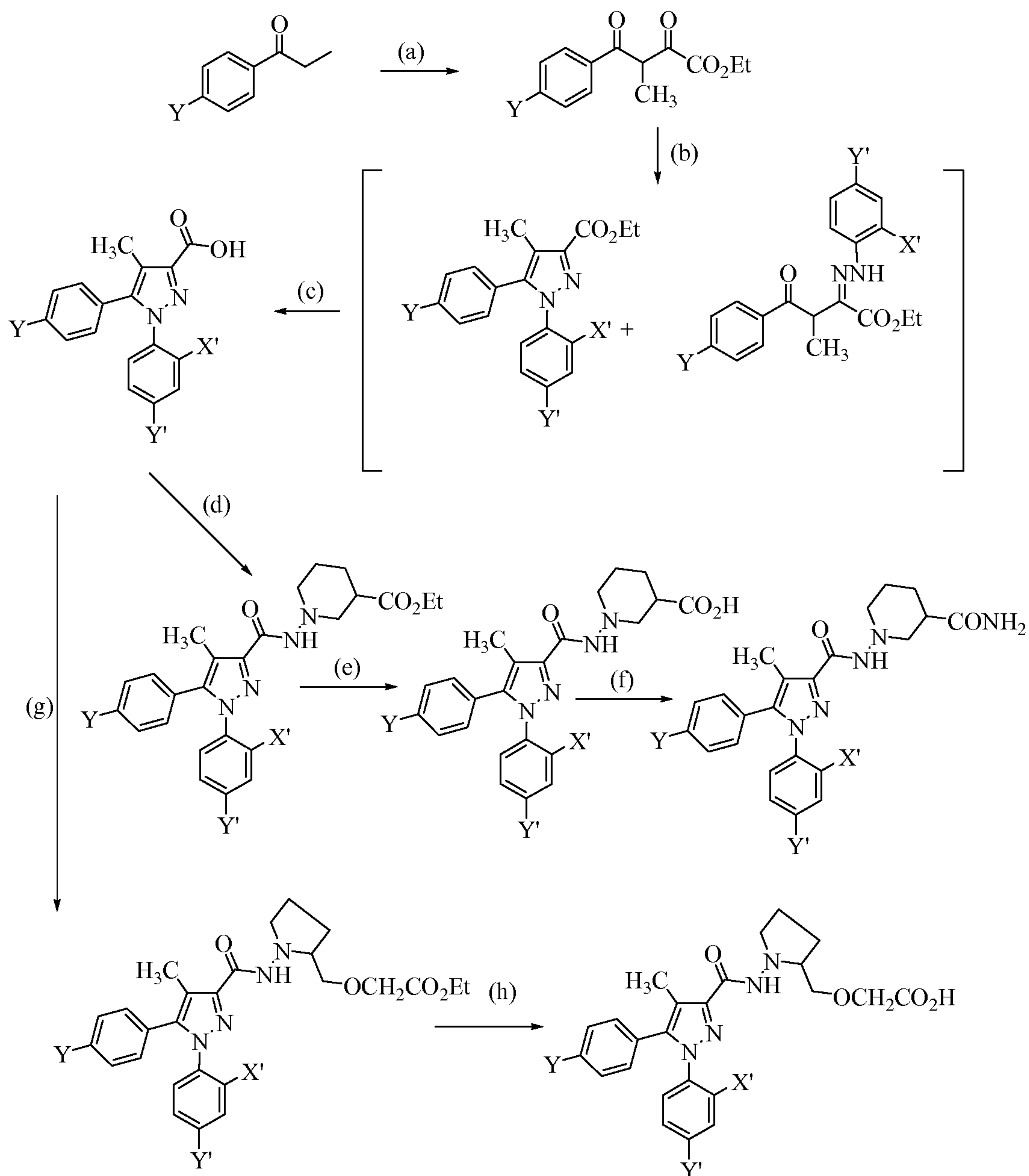
Scheme 1
