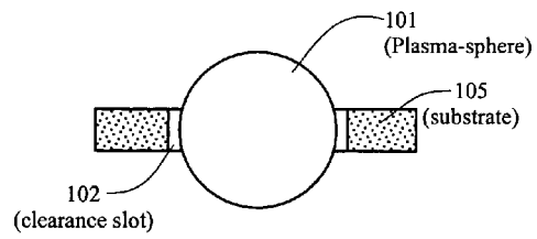
Figure 1B Section View A-A
