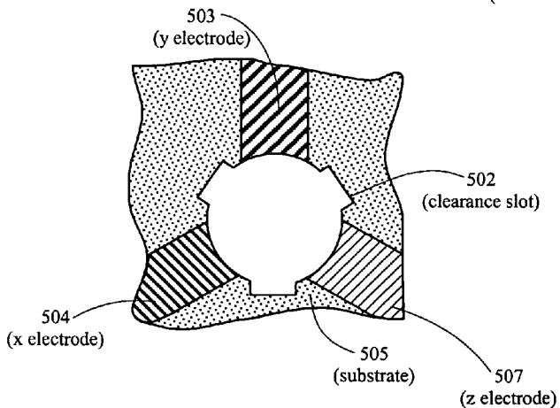
Figure 5C Top View Without the Plasma-disc
