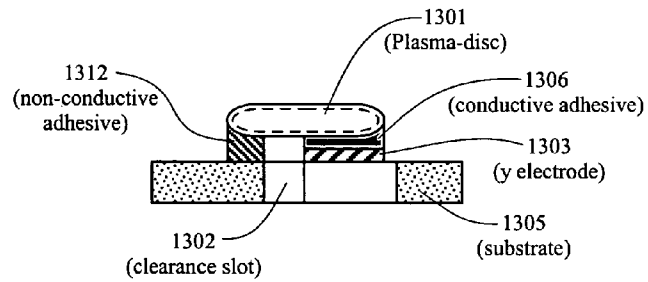
Figure 13B Section View A-A
