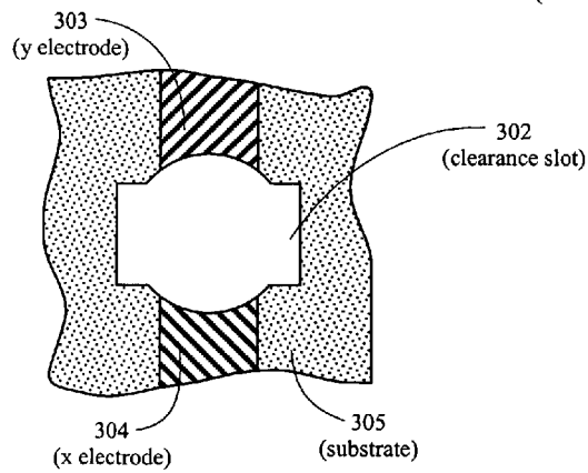
Figure 3C Top View Without the Plasma-disc
