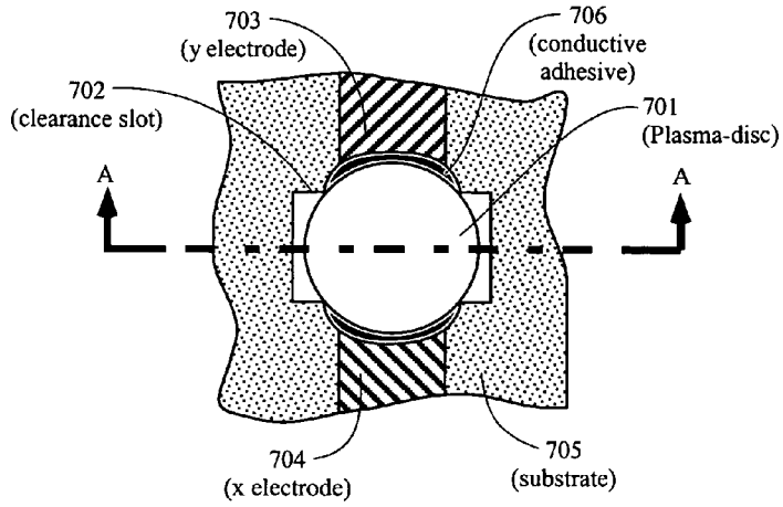
Figure 7A Top View
