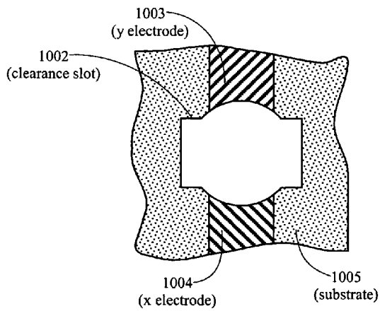
Figure 10C Top View Without the Plasma-dome
