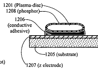
Figure 12C Section View B-B
