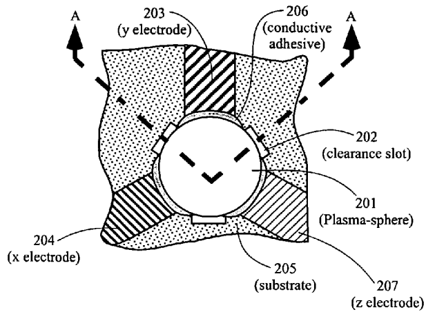
Figure 2A Top View
