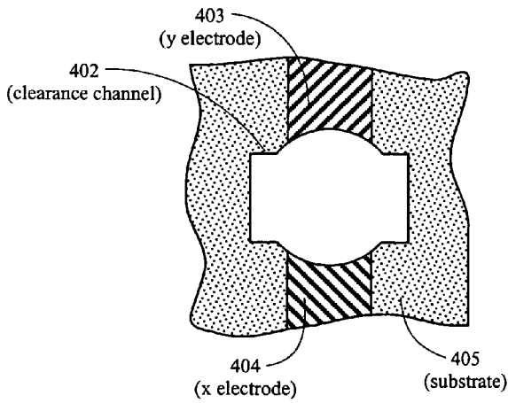
Figure 4C Top View Without the Plasma-disc
