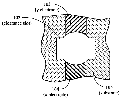
Figure 1C Top View Without the Plasma-sphere
