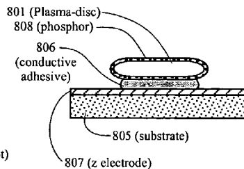
Figure 8C Section View B-B
