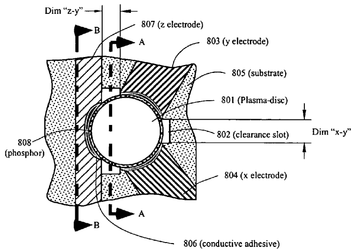
Figure 8A Top View
