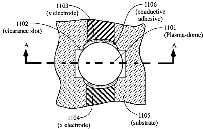
Figure 11A Top View
