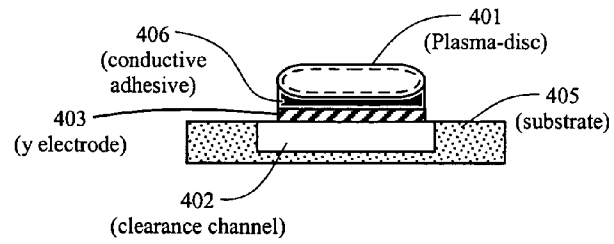
Figure 4B Section View A-A
