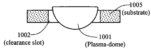
Figure 10B Section View A-A
