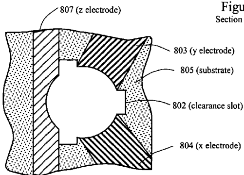
Figure 8D Top View Without the Plasma-disc
