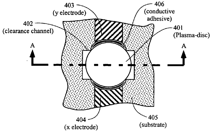
Figure 4A Top View
