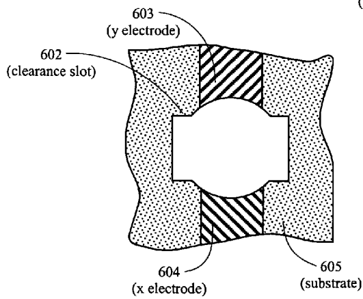
Figure 6C Top View Without the Plasma-sphere
