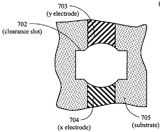
Figure 7C Top View Without the Plasma-disc
