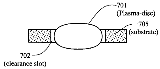
Figure 7B Section View A-A
