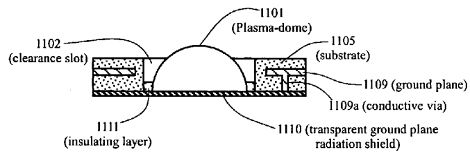
Figure 11B Section View A-A
