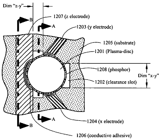
Figure 12A Top View
