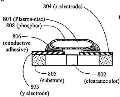
Figure 8B Section View A-A
