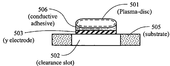
Figure 5B Section View A-A
