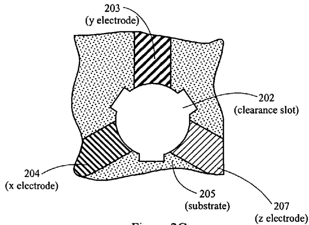
Figure 2C Top View Without the Plasma-sphere
