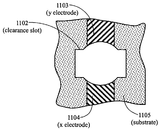
Figure 11C Top View Without the Plasma-dome
