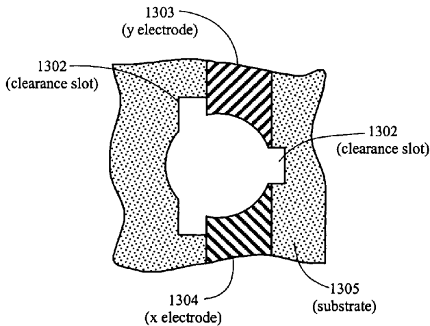
Figure 13C Top View Without the Plasma-disc
