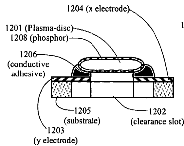
Figure 12B Section View A-A
