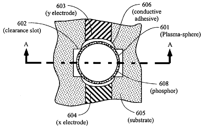
Figure 6A Top View
