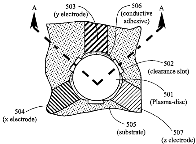
Figure 5A Top View
