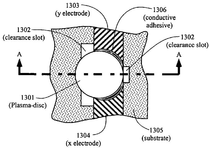
Figure 13A Top View
