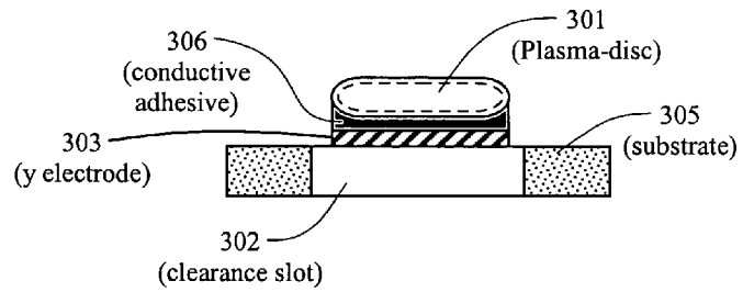
Figure 3B Section View A-A
