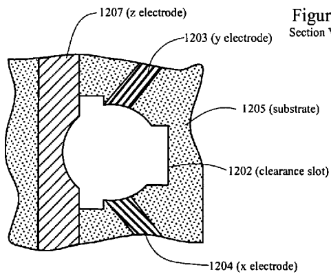
Figure 12D Top View Without the Plasma-disc
