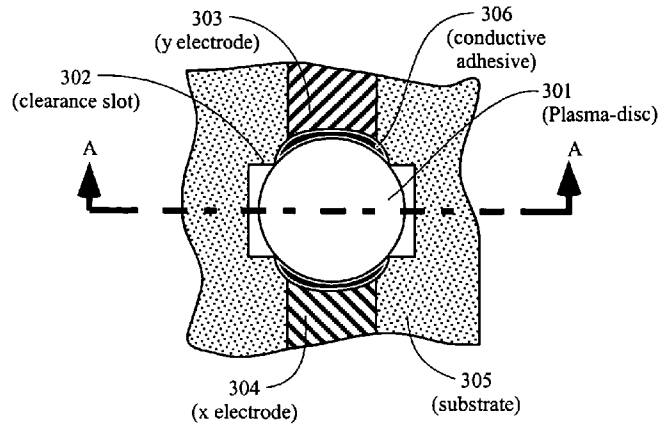
Figure 3A Top View
