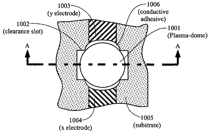
Figure 10A Top View
