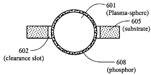
Figure 6B Section View A-A
