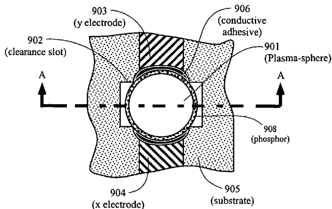
Figure 9A Top View
