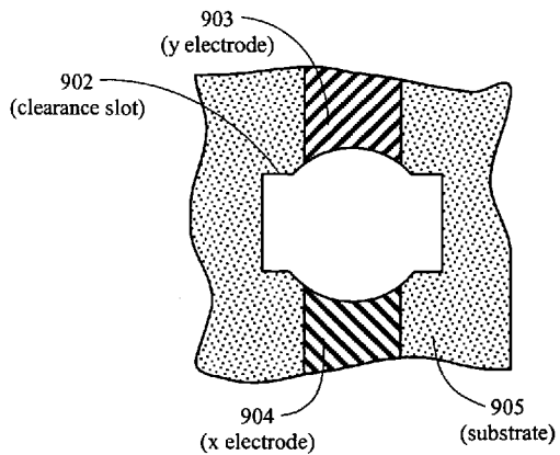
Figure 9C Top View Without the Plasma-sphere
