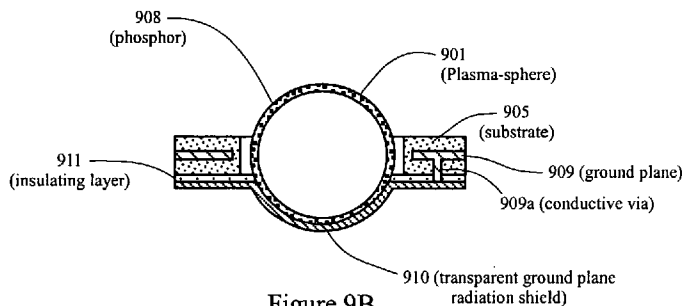
Figure 9B Section View A-A
