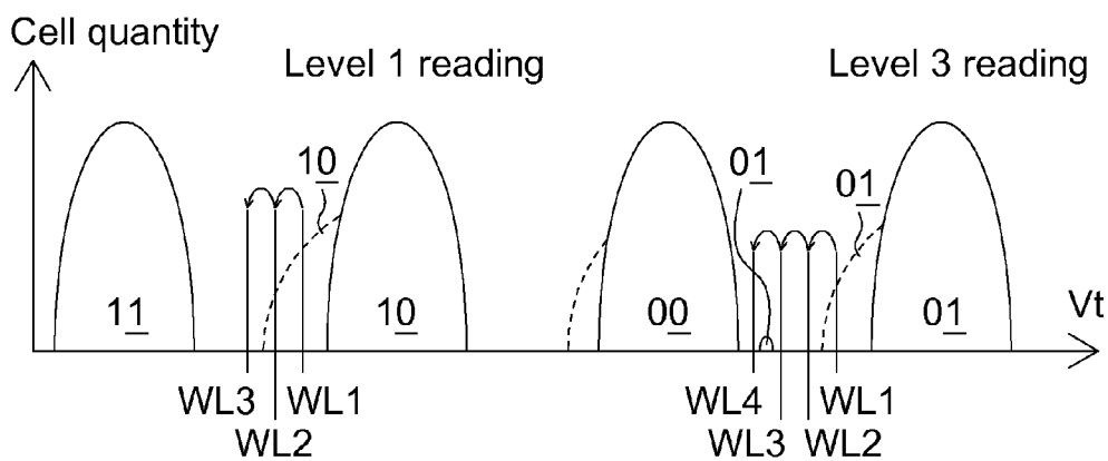
FIG. 6A(PRIOR ART)
