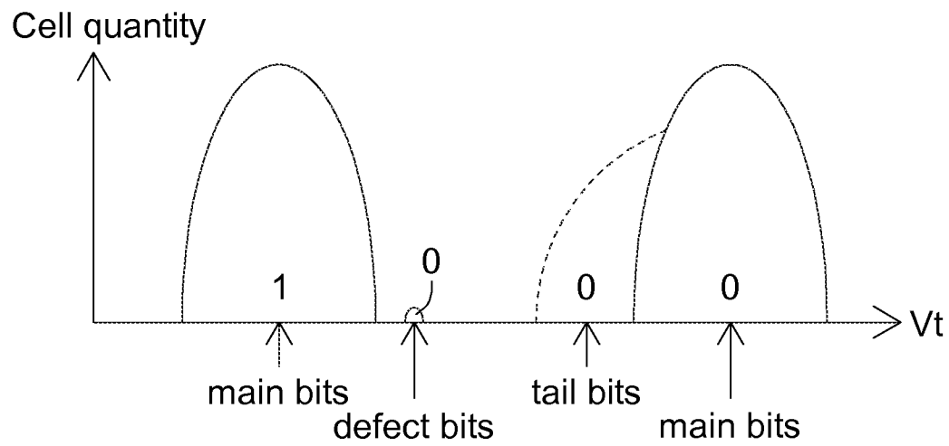
FIG. 3(PRIOR ART)
