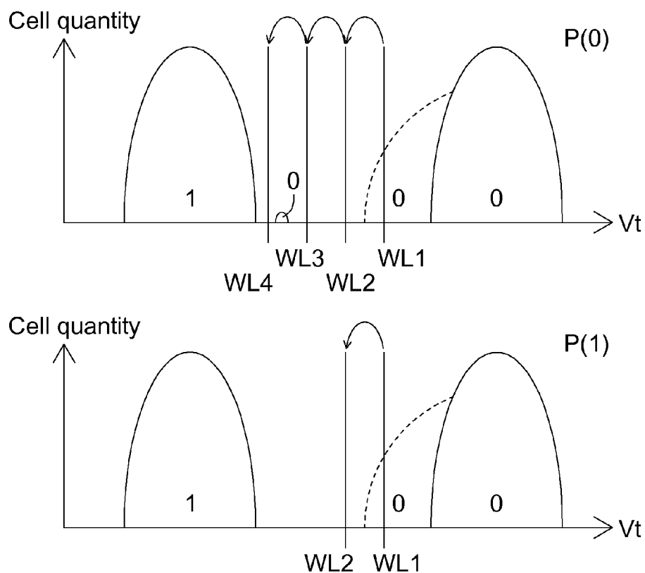
FIG. 5(PRIOR ART)
