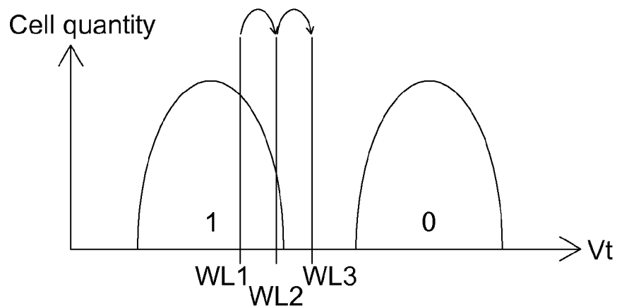
FIG. 2A(PRIOR ART)
