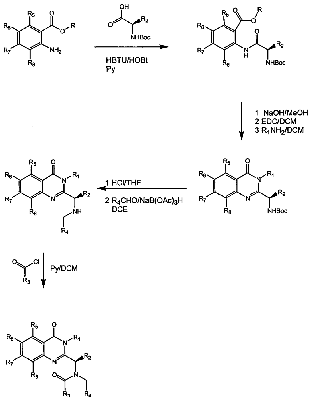
Figure 4: Asymmetric Synthesis
