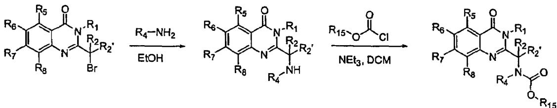
Figure 5c: Urea Synthesis
