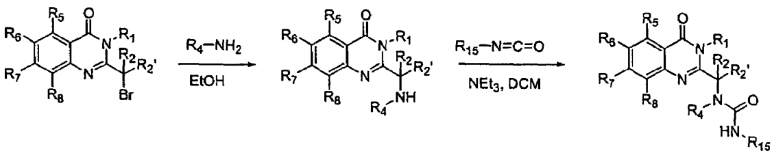
Figure 5d: Primary and Secondary Amine R_4 Synthesis
