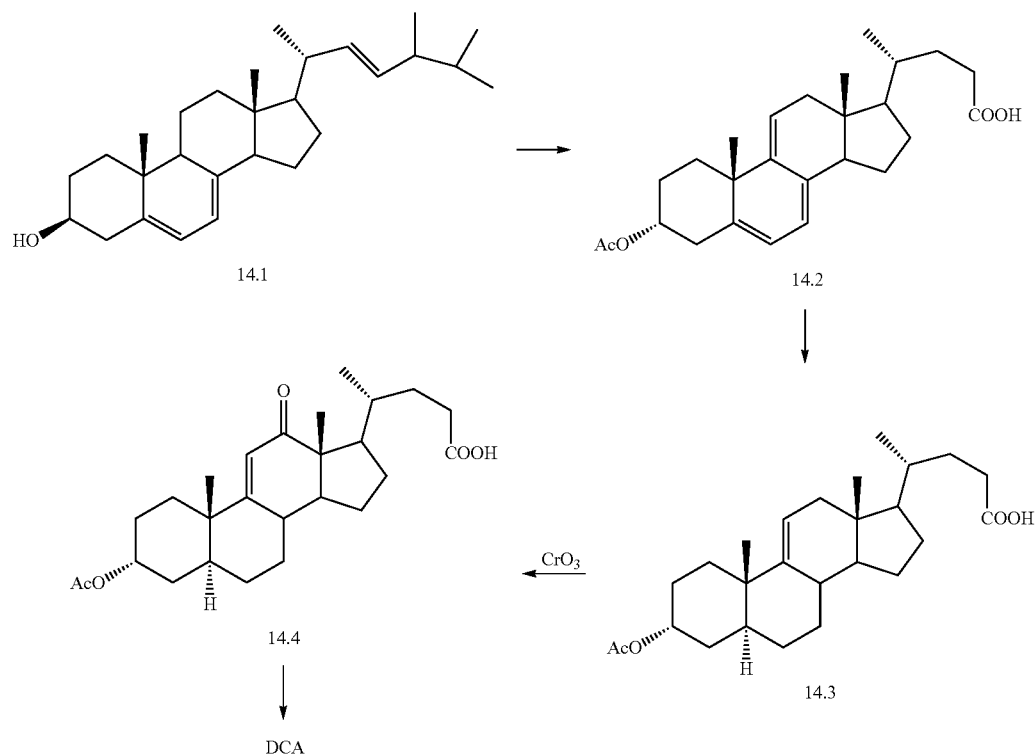
Scheme 14. Triene formation from Ergosterol
