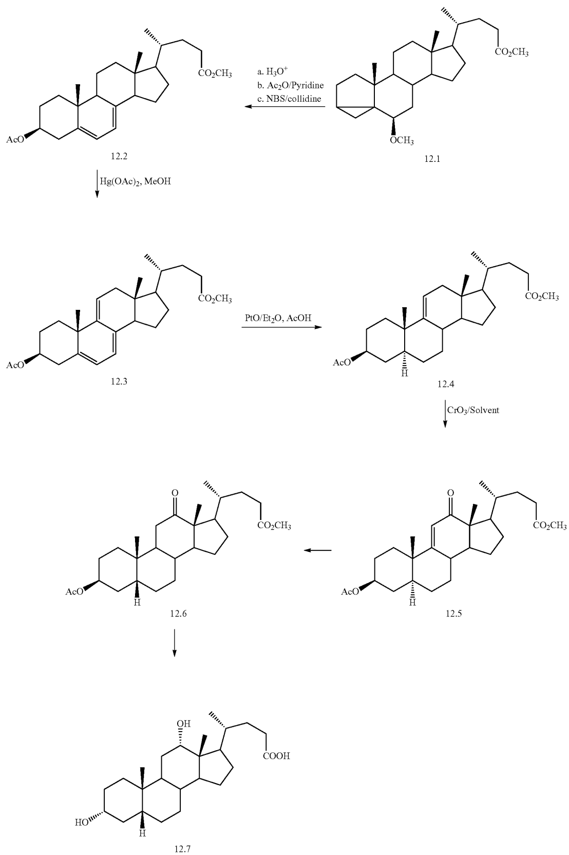
Scheme 12. Triene formation and allylic oxidation
