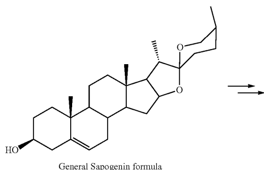
Scheme 10B. Synthetic route from saponin.
