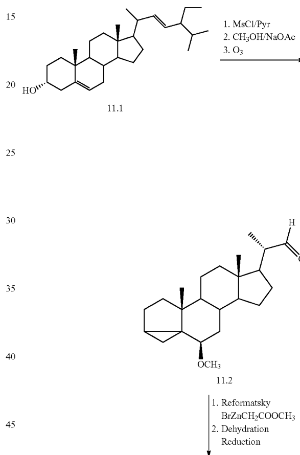
Scheme 11. Ozonolysis of i-steroid and side chain reduction
