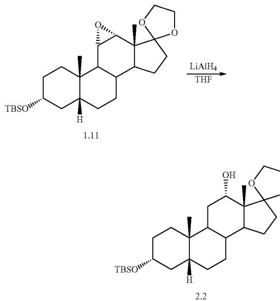
Scheme 3. Stereoselective Reduction of C 11 -C 12 epoxide.
