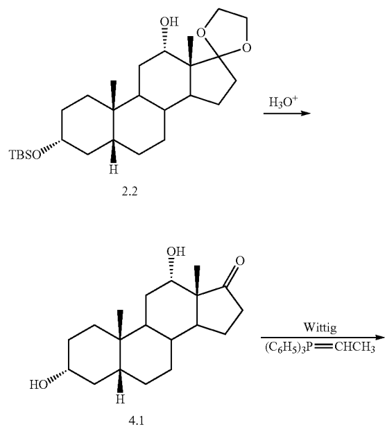
Scheme 4. Deprotection and Wittig Reaction
