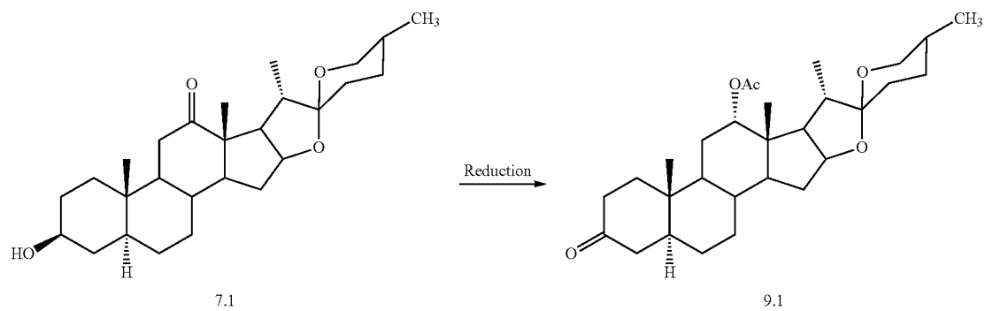
Scheme 9. Dithioethane route to 3-keto-4-ene
