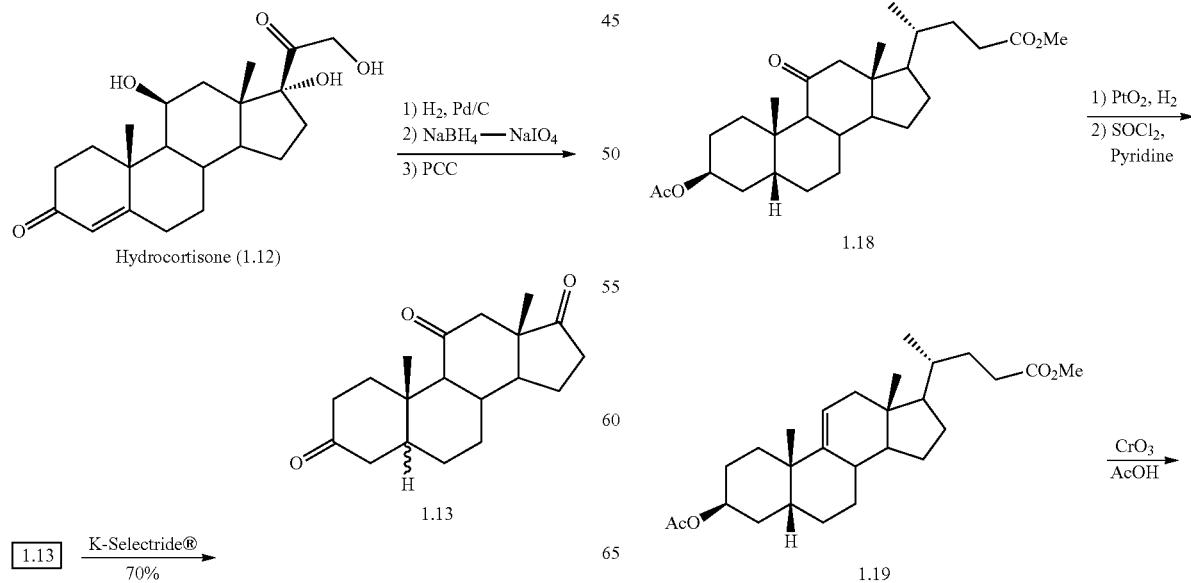
Scheme 1B. Synthesis of DCA from Hydrocortisone
