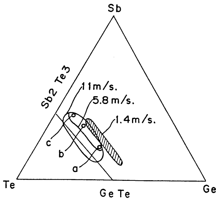
Fig. 17 PRIOR ART
