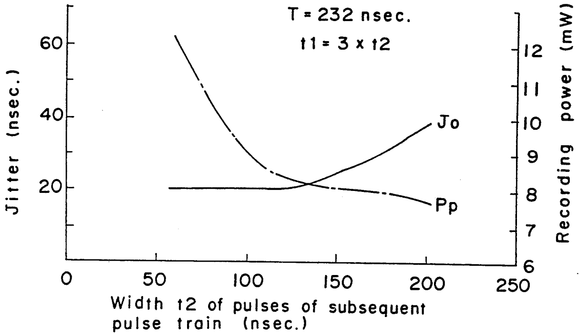
Fig. 17 PRIOR ART
