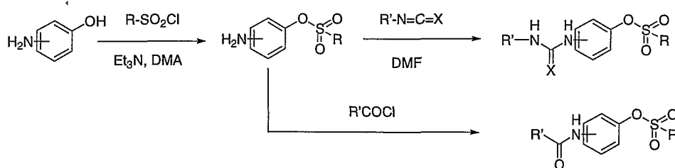
Scheme V
