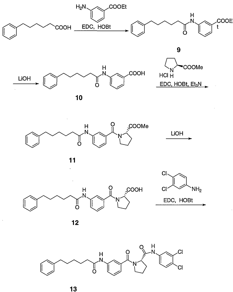
Scheme XIX
