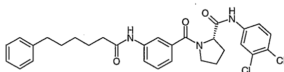
Compound # 36
