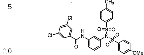
Compound # 3
