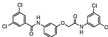
Compound # 24
