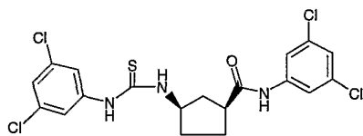
Compound # 17
