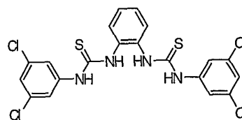
Compound # 28
