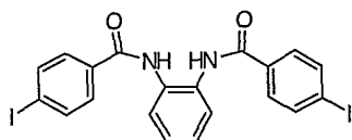
Compound # 29
