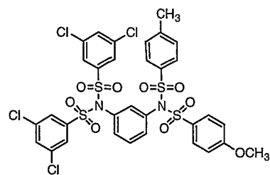
Compound # 4
