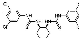
Compound # 15
