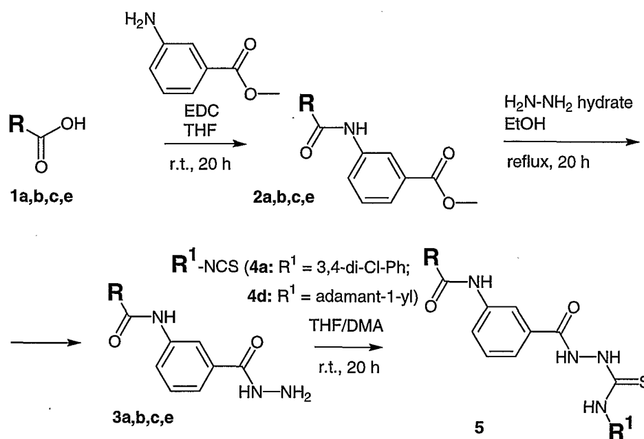
Scheme XI
