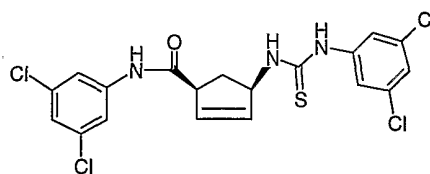
Compound # 18
