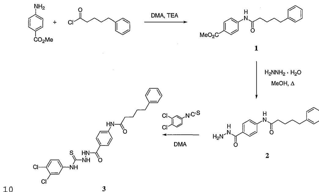
Scheme XVI
