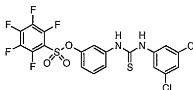
Compound # 22
