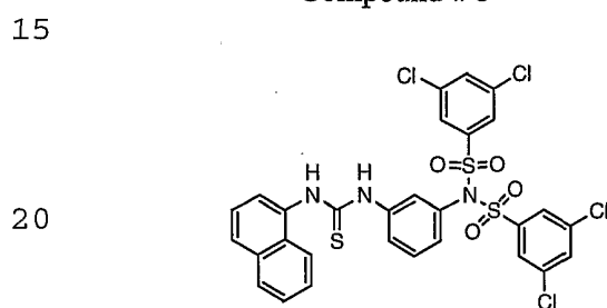
Compound # 5
