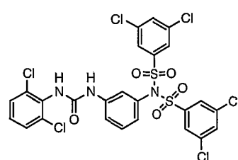
Compound # 6
