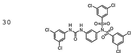
Compound # 7
