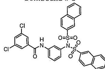
Compound # 8
