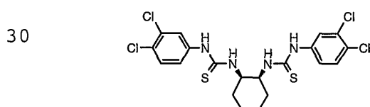
Compound # 14
