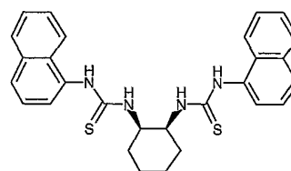
Compound # 11
