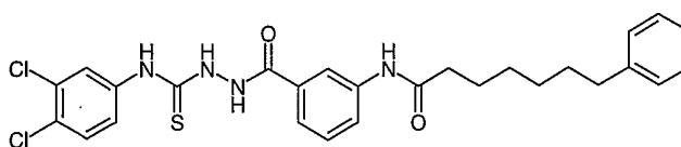
Compound # 37
