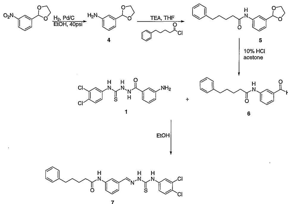
Scheme XIV
