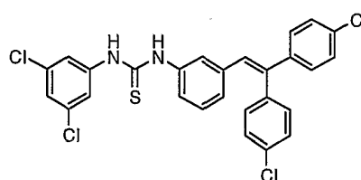
Compound # 20
