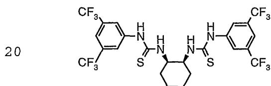
Compound # 12
