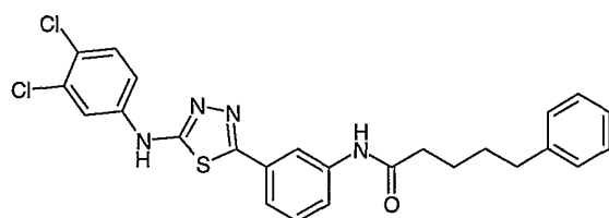
Compound # 40A
