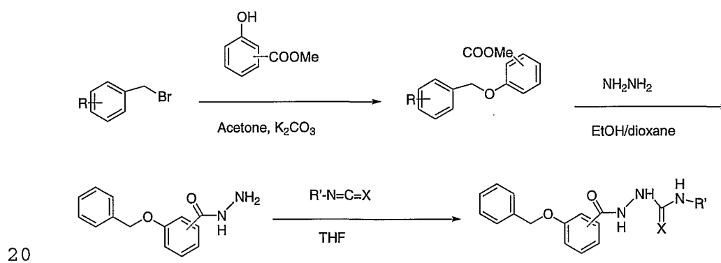
Scheme VIII
