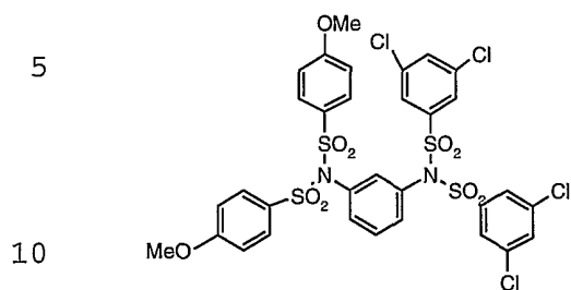
Compound # 10
