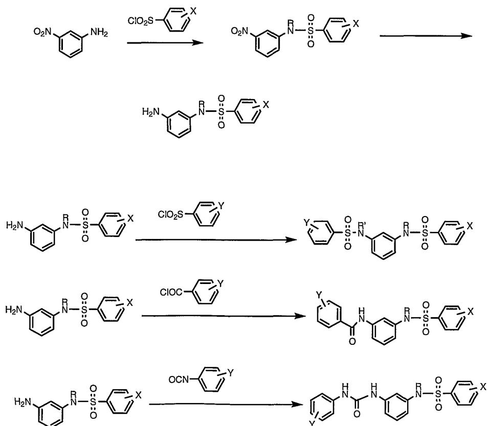
Scheme I
