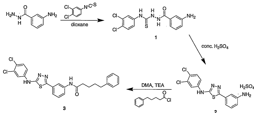
Scheme XIII
