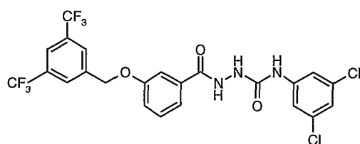
Compound # 23
