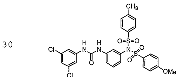
Compound # 1
