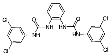
Compound # 27
