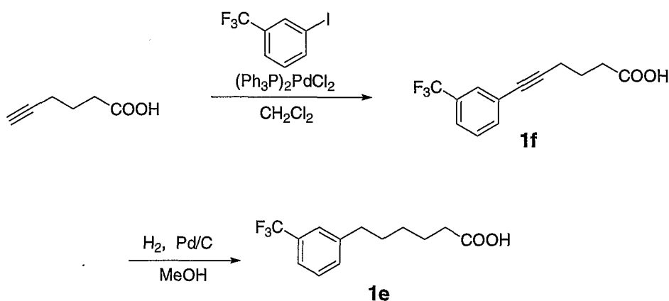
Scheme X
