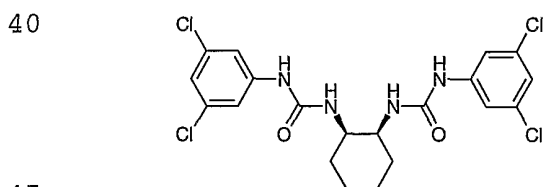
Compound # 15a
