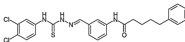
Compound # 39
