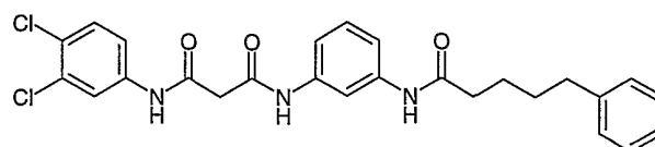
Compound # 42
