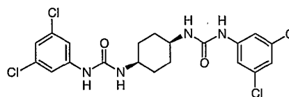
Compound # 16
