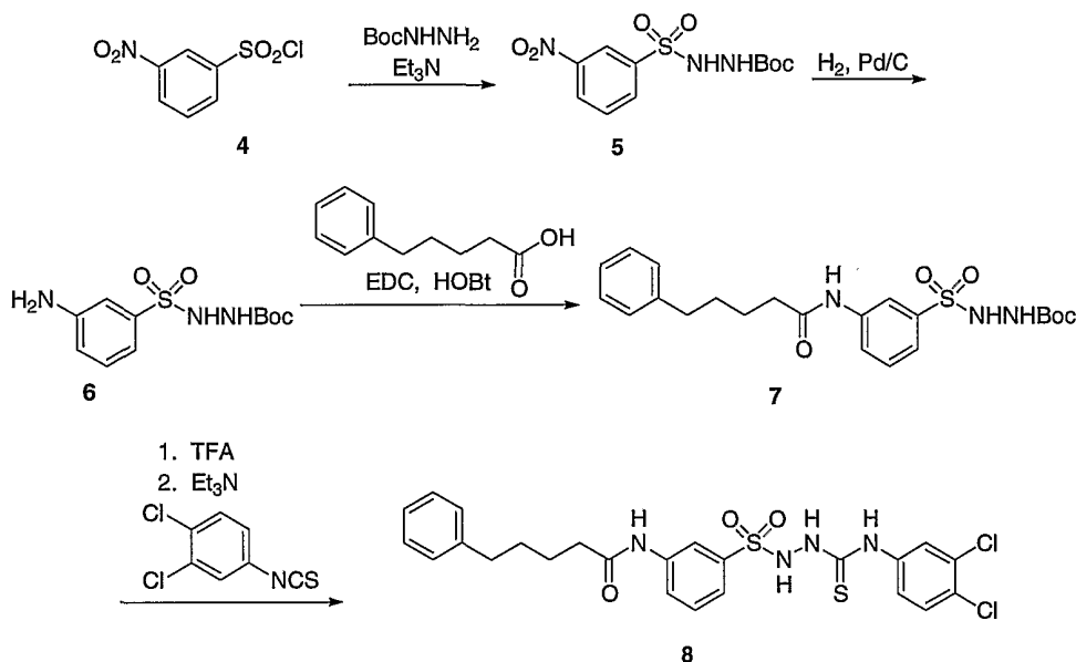
Scheme XVIII
