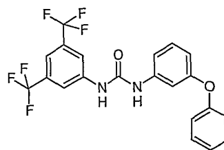
Compound # 26
