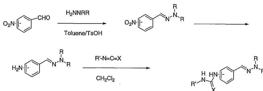
Scheme VII
