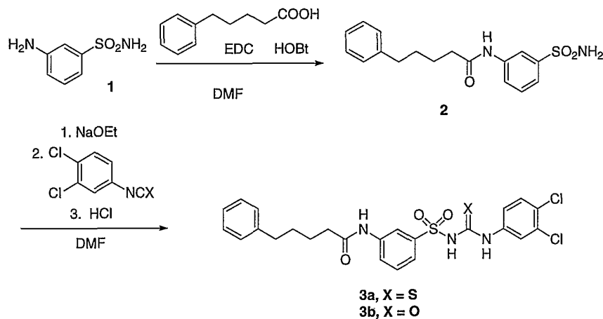
Scheme XVII
