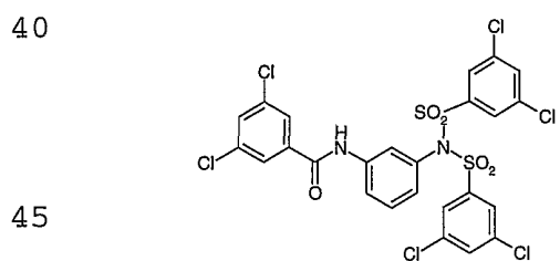
Compound # 8a
