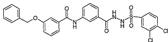
Compound # 31
