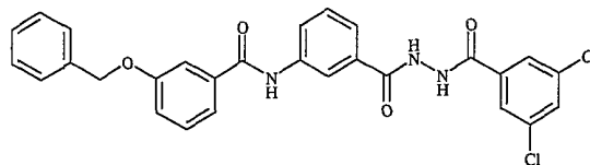
Compound # 30
