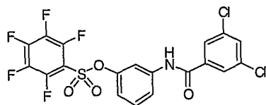
Compound # 25
