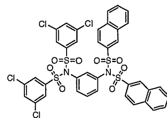
Compound # 9
