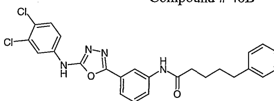
Compound # 40B
