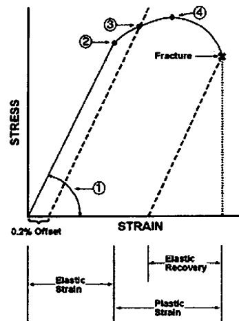
Fig. 17 (Typical stress versus strain curve of a material)
