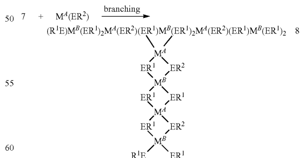
REACTION SCHEME 5:
