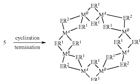
REACTION SCHEME 7:
