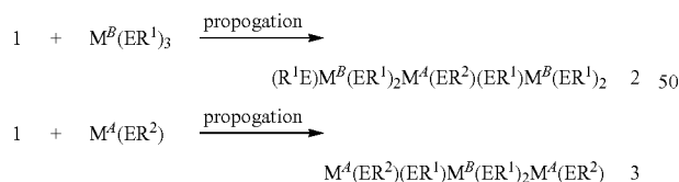
REACTION SCHEME 2:
