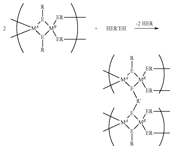
REACTION SCHEME 14
