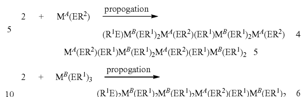
REACTION SCHEME 3:
