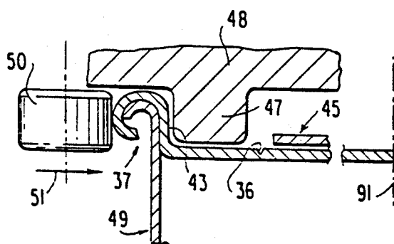
FIG. 3 PRIOR ART
