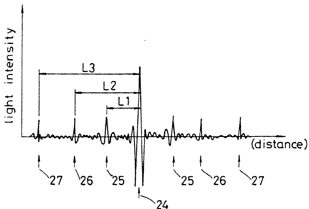
Fig.13 PRIOR ART
