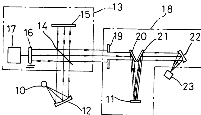
Fig. 11 PRIOR ART
