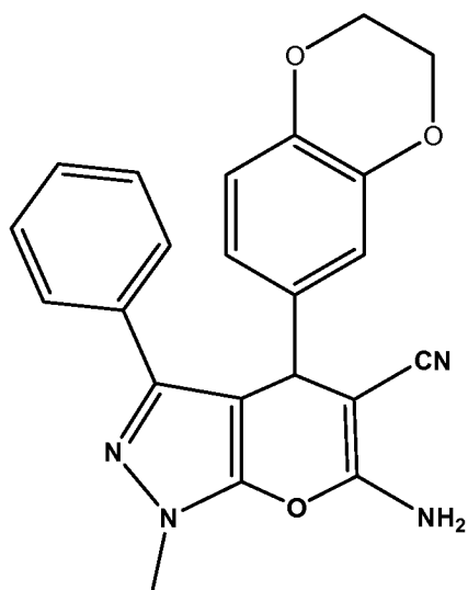
6-amino-4-(2,3-dihydrobenzo[b][1,4]dioxin-6-yl)-1-methyl-3-phenyl-1,4-dihydropyrano [2,3-c]pyrazole-5-carbonitrile.
