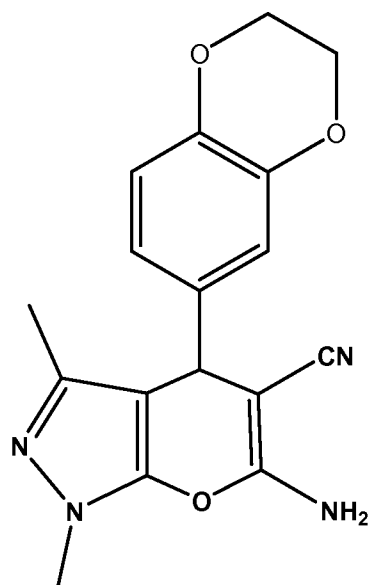
6-amino-1-methyl-3-phenyl-4-(4-(trifluoromethoxy)phenyl)-1,4-dihydropyrano [2,3-c]pyrazole-5-carbonitrile,
