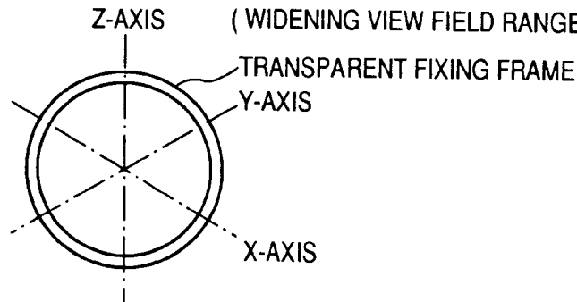
FIG. 4B TYPE USING RING-SHAPED (LARGE NUMBER OF) PIEZOELECTRIC ELEMENTS
