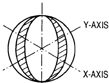
FIG. 4B TYPE USING RING-SHAPED (LARGE NUMBER OF) PIEZOELECTRIC ELEMENTS
