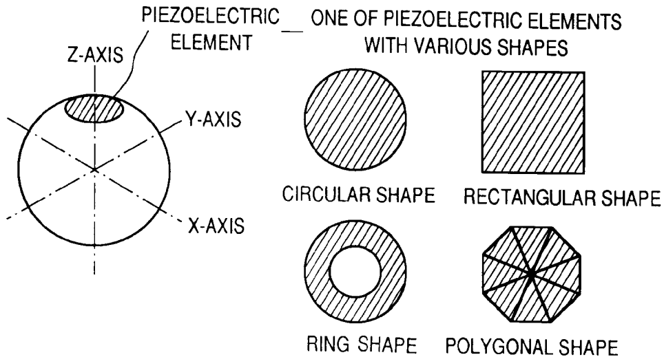
FIG. 4D TYPE USING ONE PIEZOELECTRIC ELEMENT
