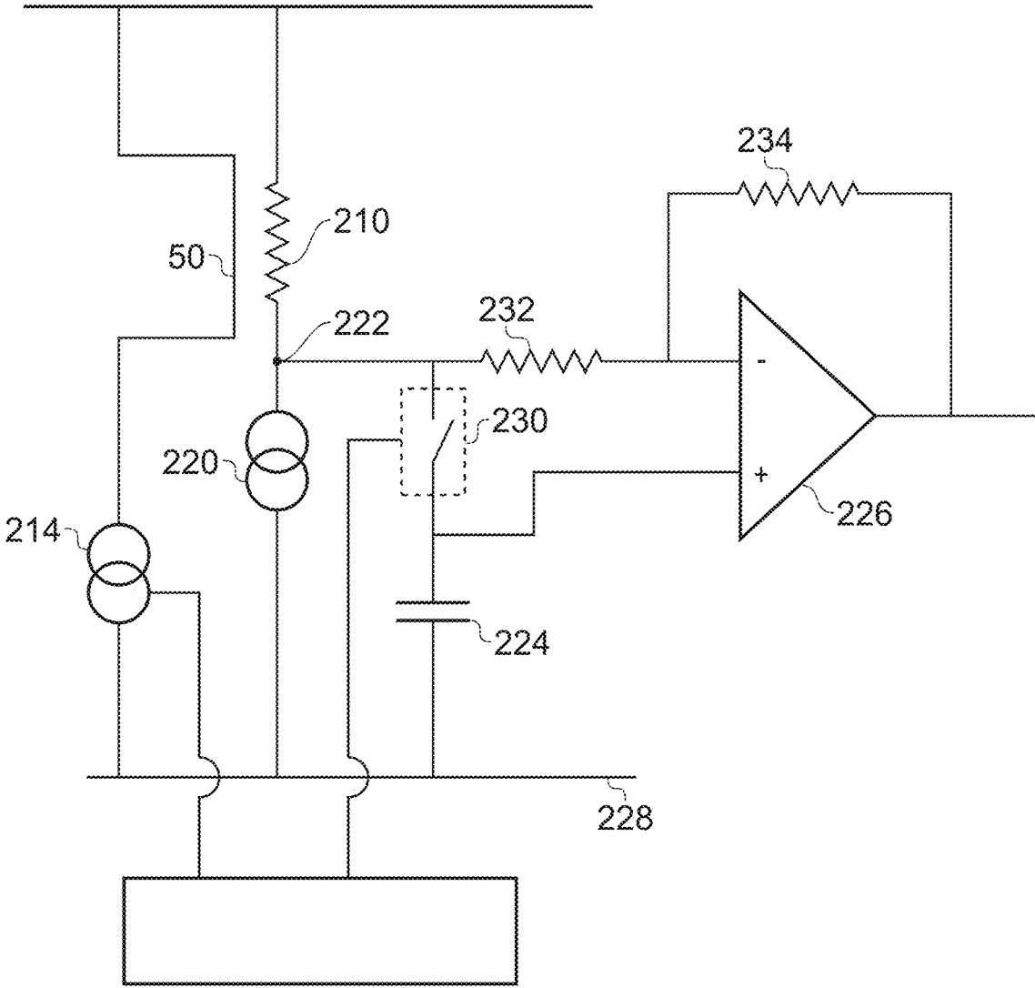
FIG. 19 (PRIOR ART)
