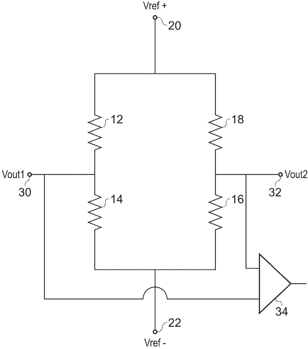
FIG. 2 (PRIOR ART)
