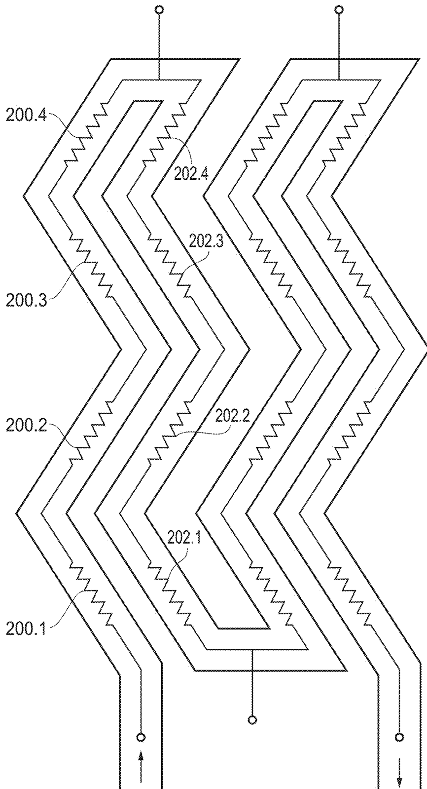
FIG. 18 (PRIOR ART)
