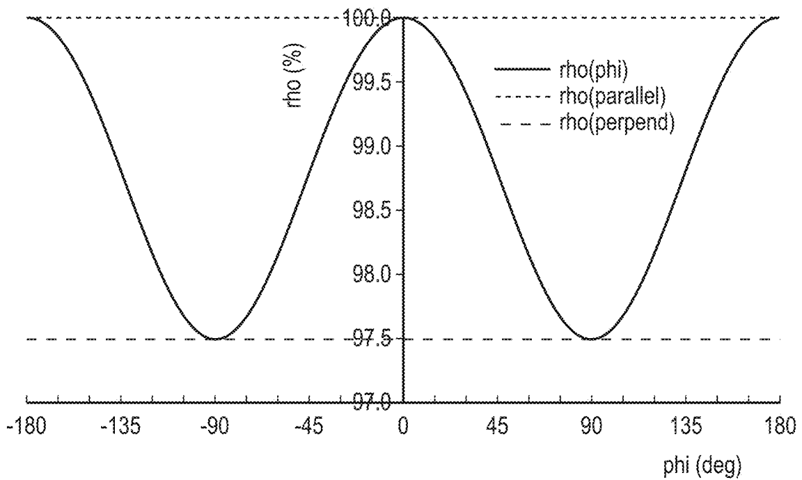
FIG. 6 (PRIOR ART)
