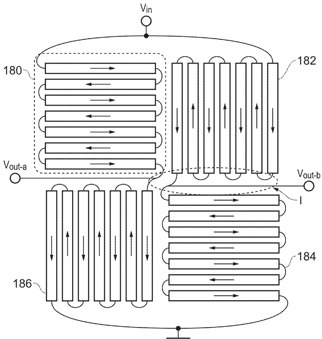
FIG. 14 (PRIOR ART)
