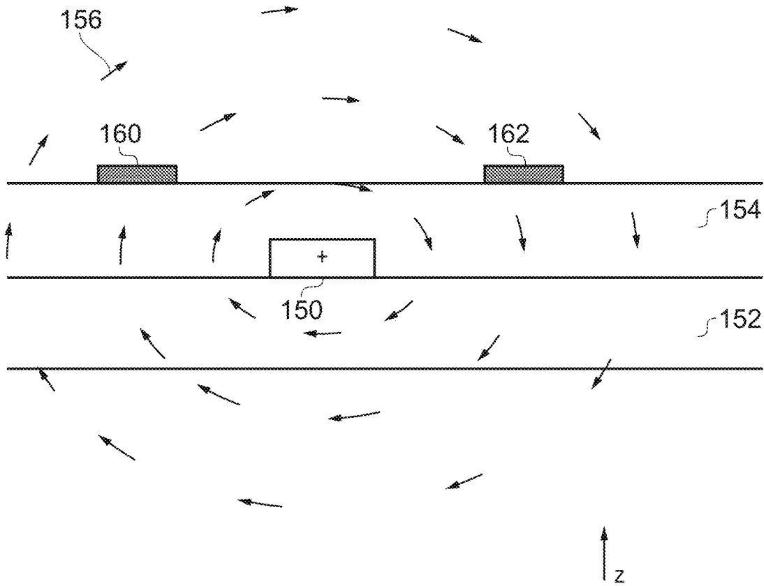
FIG. 12 (PRIOR ART)
