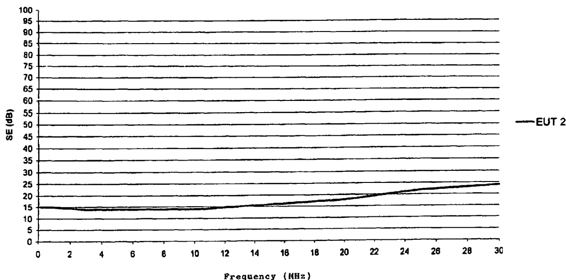
Measurement SE - ELECTRIC Field(0,1 - 30) MHz
