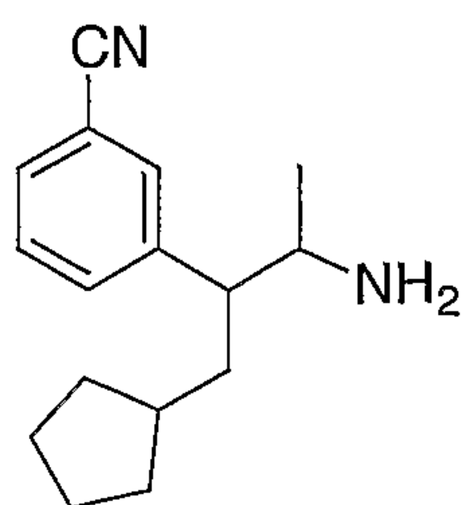
2-(3-Cyanophenyl)-3-cyclopentyl-1-methylpropylamine
