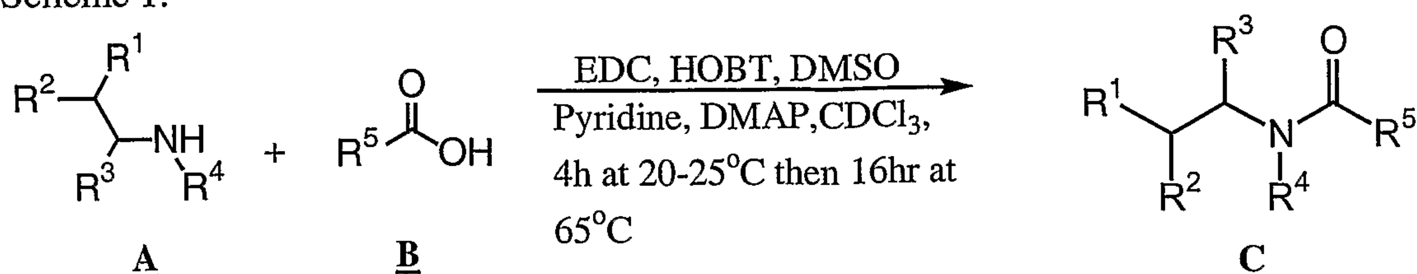
Scheme 1.
