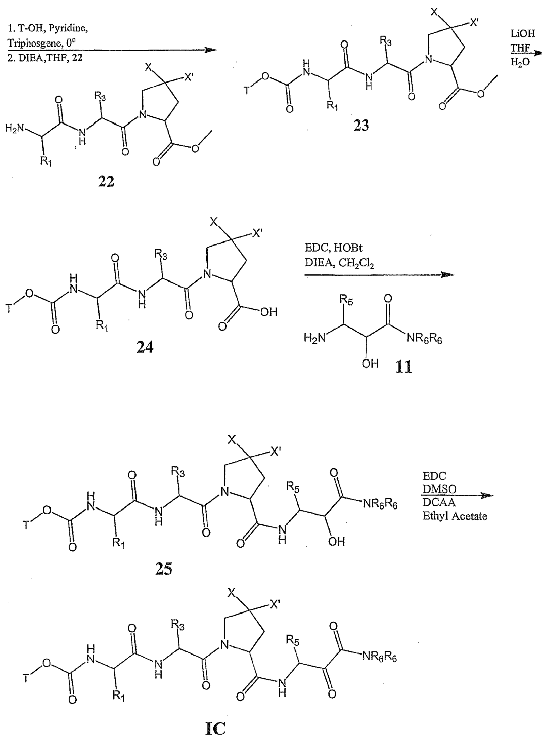
Scheme 3:
