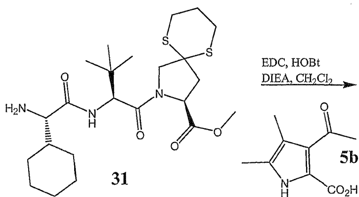
Scheme 6:
