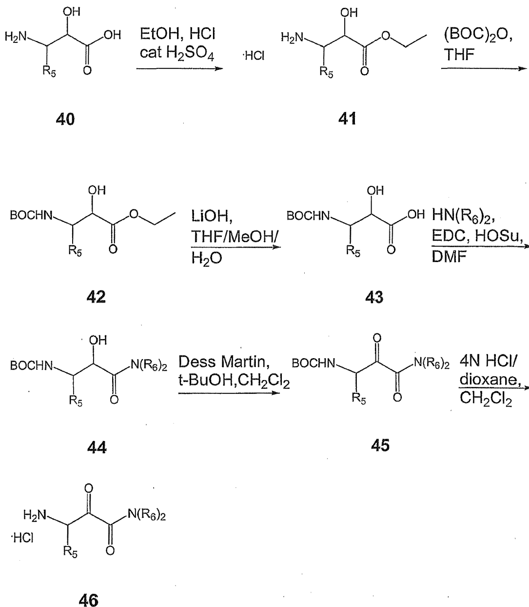
Scheme 1A:
