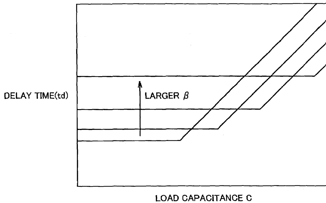
FIG.16 PRIOR ART
