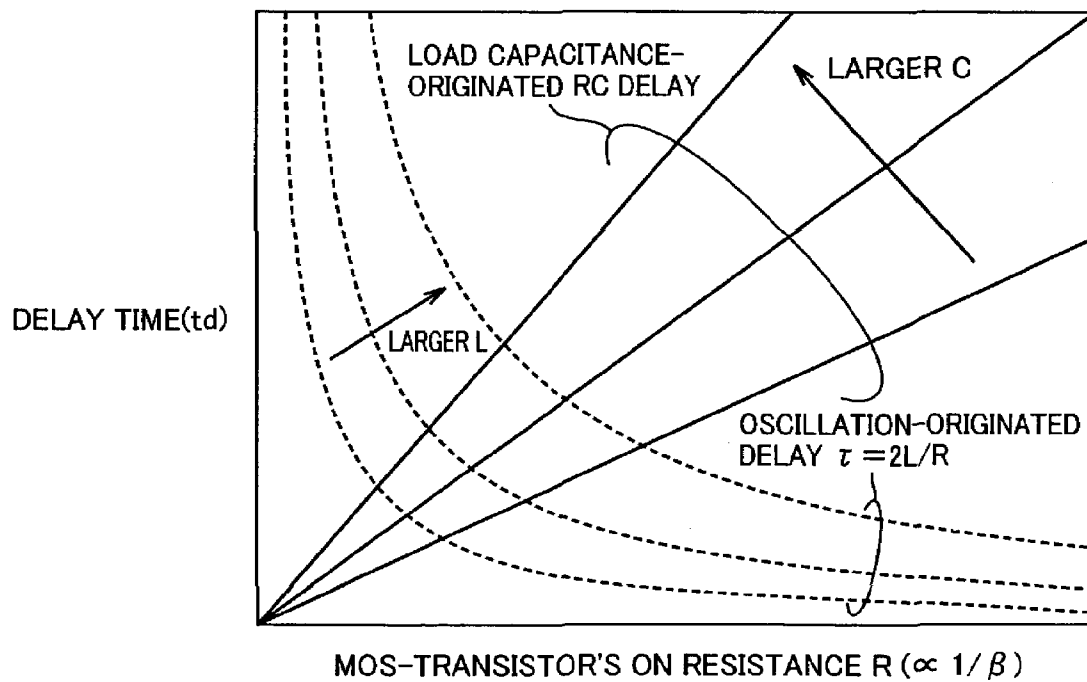
FIG. 15 PRIOR ART
