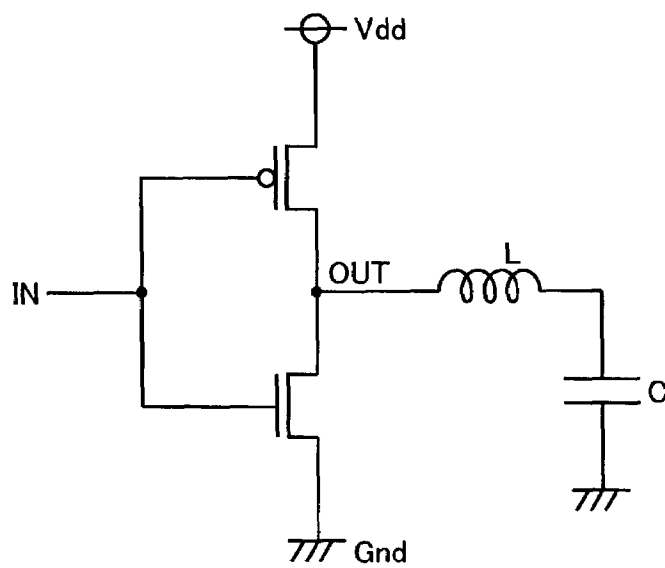
FIG.13 PRIOR ART
