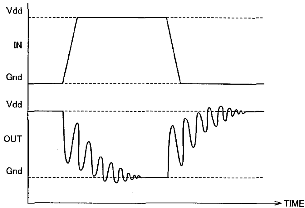
FIG. 14 PRIOR ART
