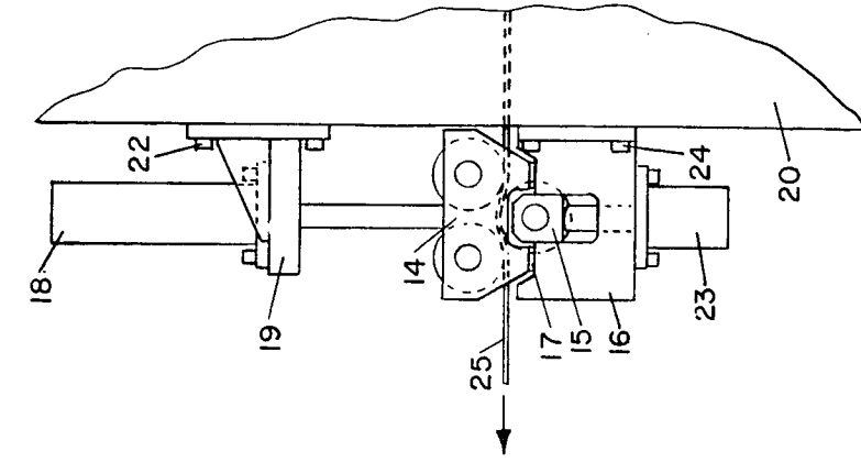
FIG. 2 (PRIOR ART)
