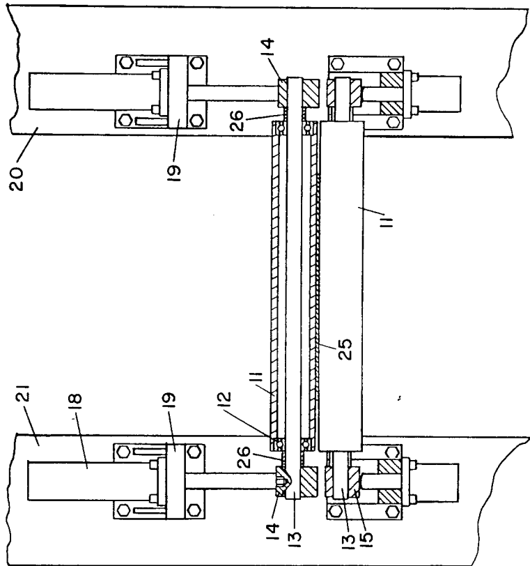
FIG. 1 (PRIOR ART)
