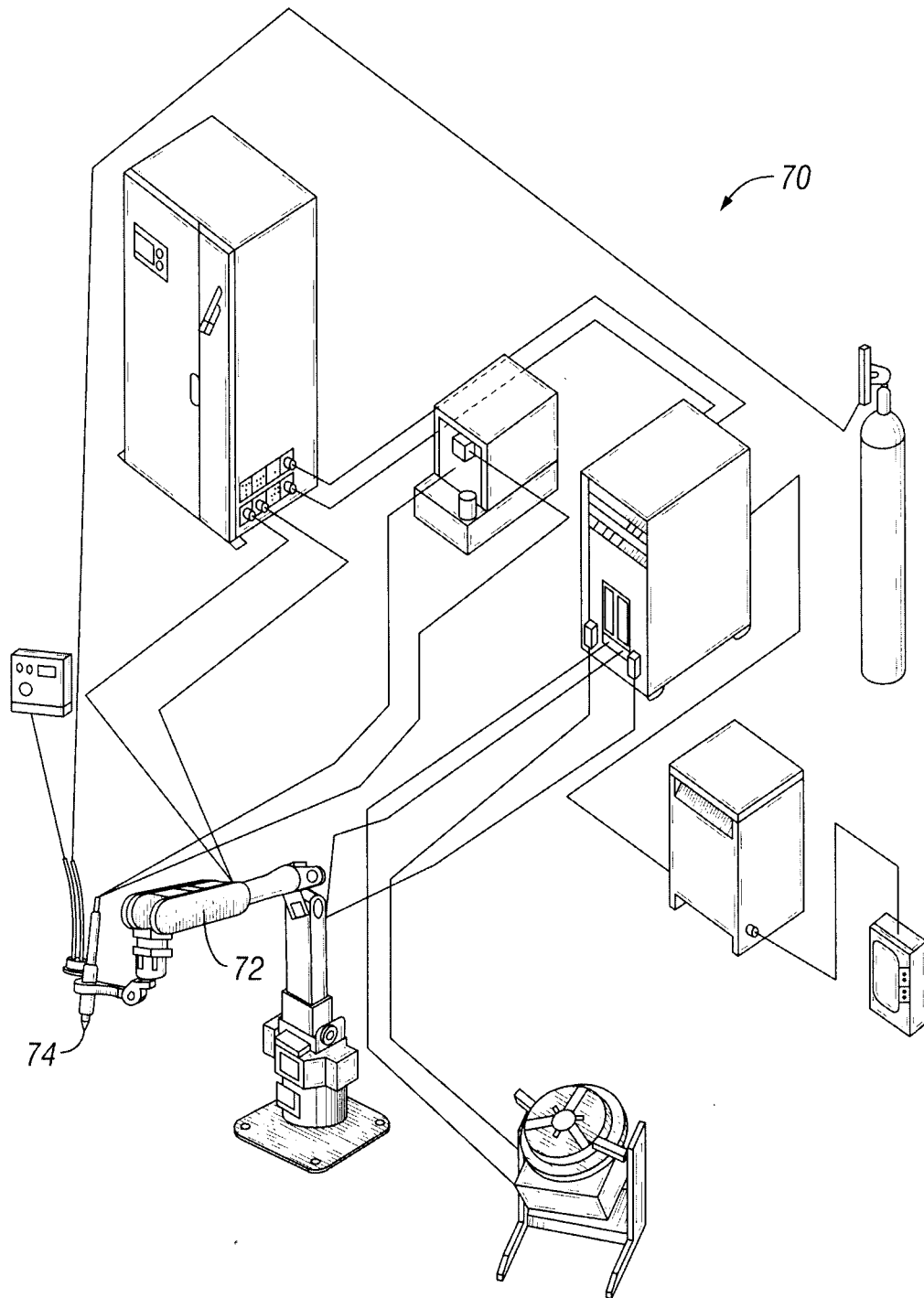
FIG. 7 (Prior Art)
