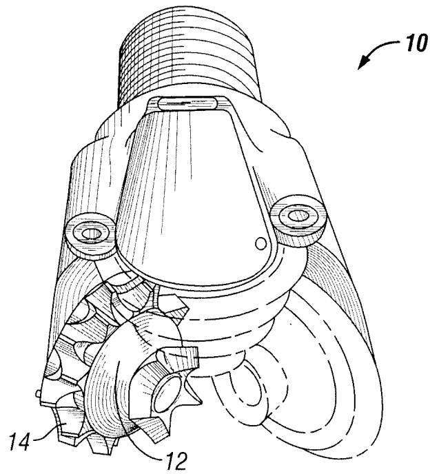
FIG. 1 (Prior Art)
