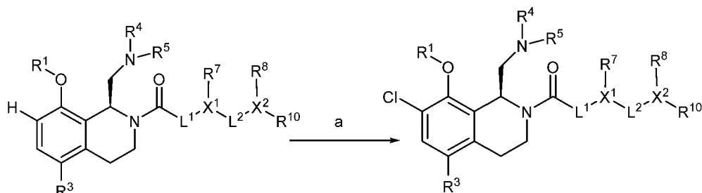
Scheme 6: a) NCS, DCM/DMF.
