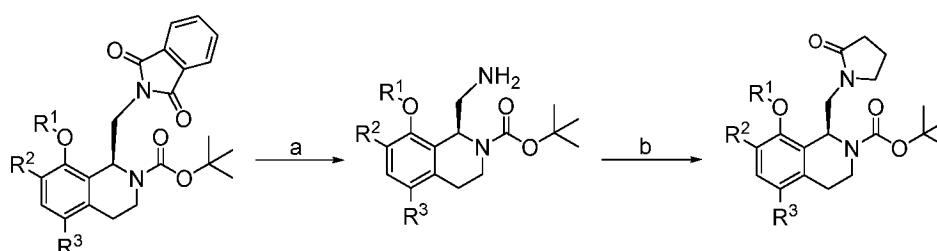
Scheme 5: a) N 2 H 4 , EtOH; b) methyl 4-bromobutanoate, Et 3 N, PhMe.
