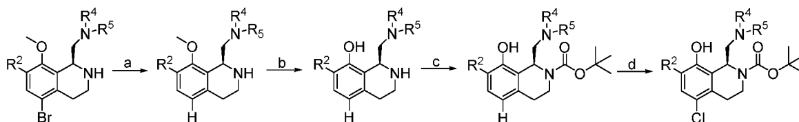
Scheme 2: a) H_2 , 10% Pd/C, THF, EtOH; b) BBr_3 , DCM; c) Boc_2O , DCM; d) NCS, DMF.
