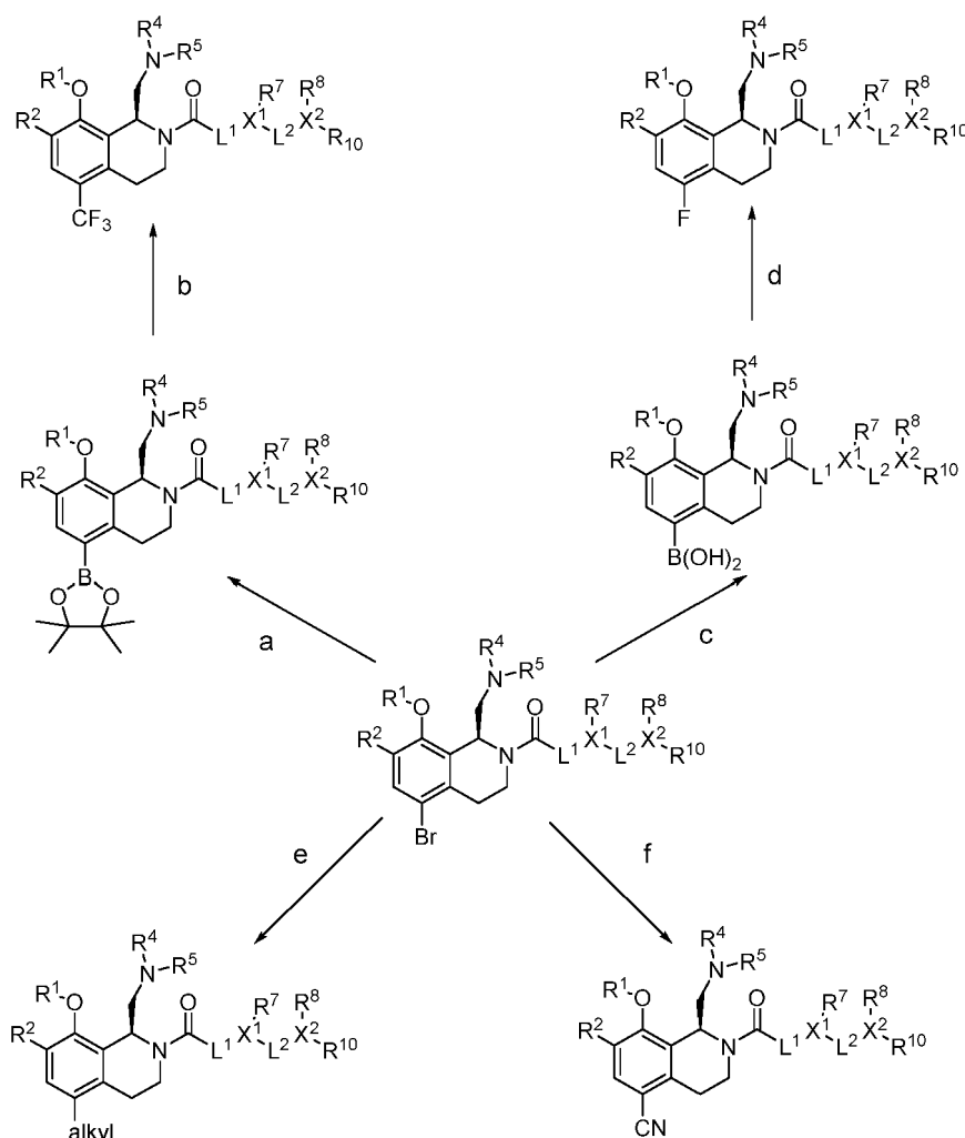
Scheme 3: a) dicyclohexyl-[2-(2,4,6-triisopropylphenyl)phenyl]phosphane, X-phos Pd, hypoboric acid; b) CF_3SO_3Ag , SelectFluor®; c) bis(pinacolato)diboron, Pd(dppf)Cl_2 ; d) potassium trimethoxy(trifluoromethyl)boranide, Cu(OAc)_2 ; e) Pd(dppf)Cl_2 , alkyl borane; f) Zn(CN)_2 , Pd(PPh_3)_4 .
