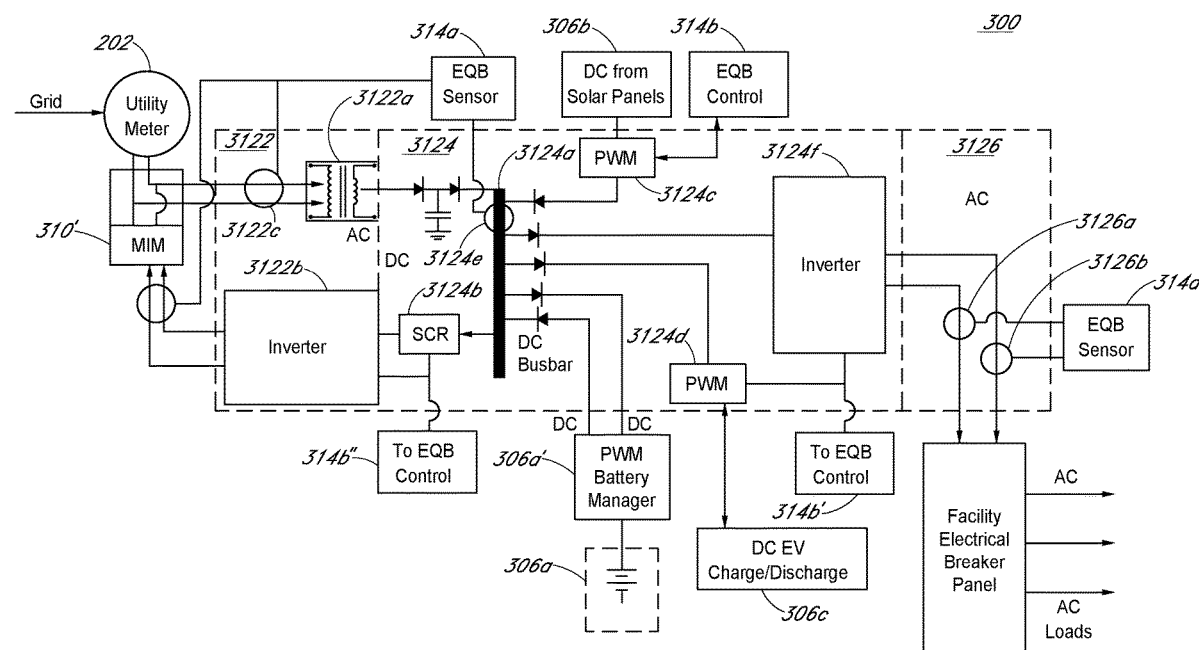
Expanded Non-Limiting View of Dynamic f_o Power Electronics Module
