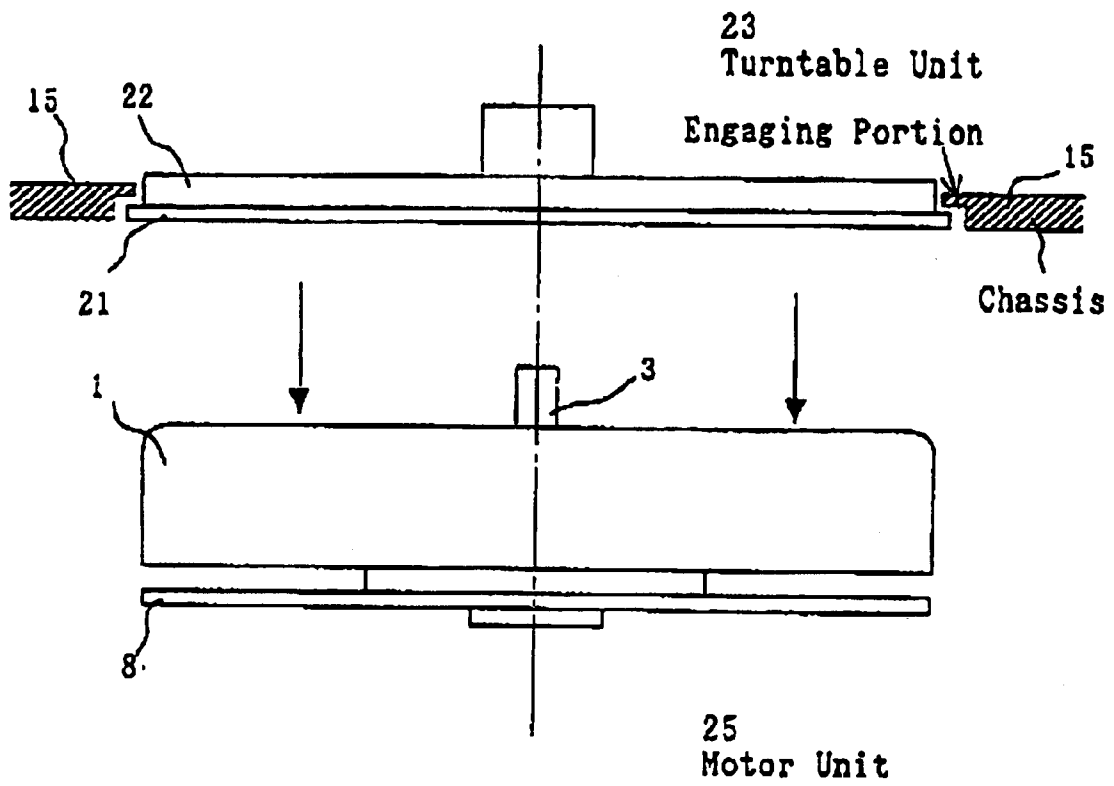
Fig.4 (PRIOR ART)
