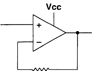
NON-INVERTING AMPLIFIER Q2
