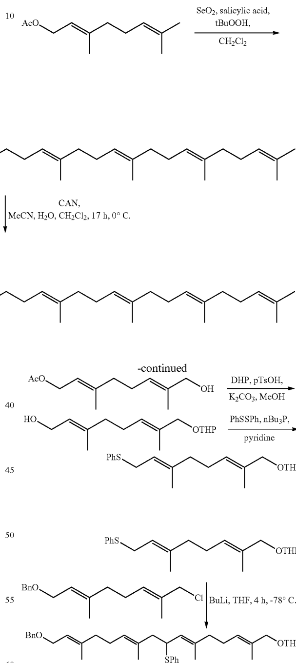
Scheme A: Synthesis of allylic thioether.
