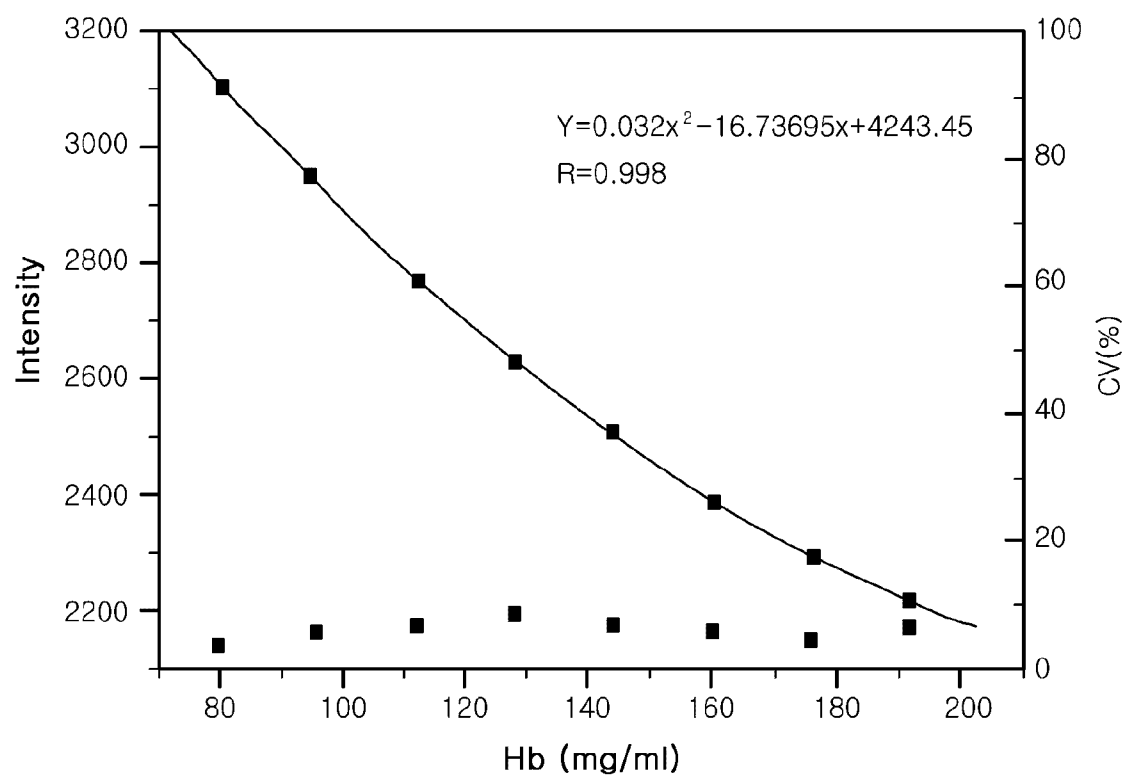
Hb standard curve using LED detection system
