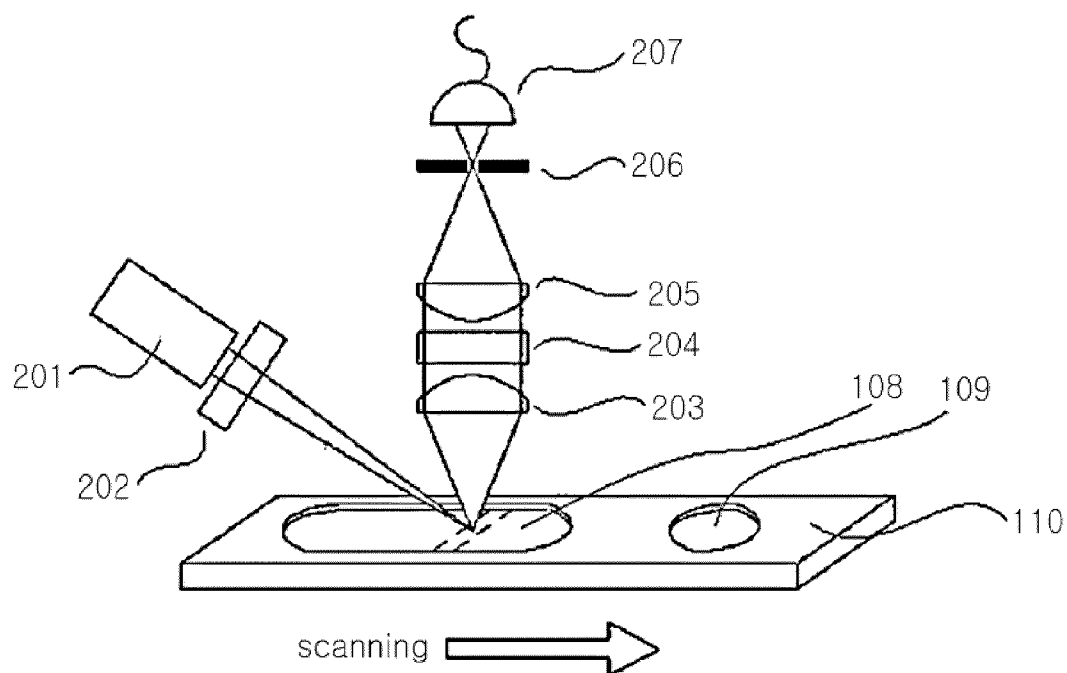
FIG. 3-A: Laser-induced epifluorescence detection device
