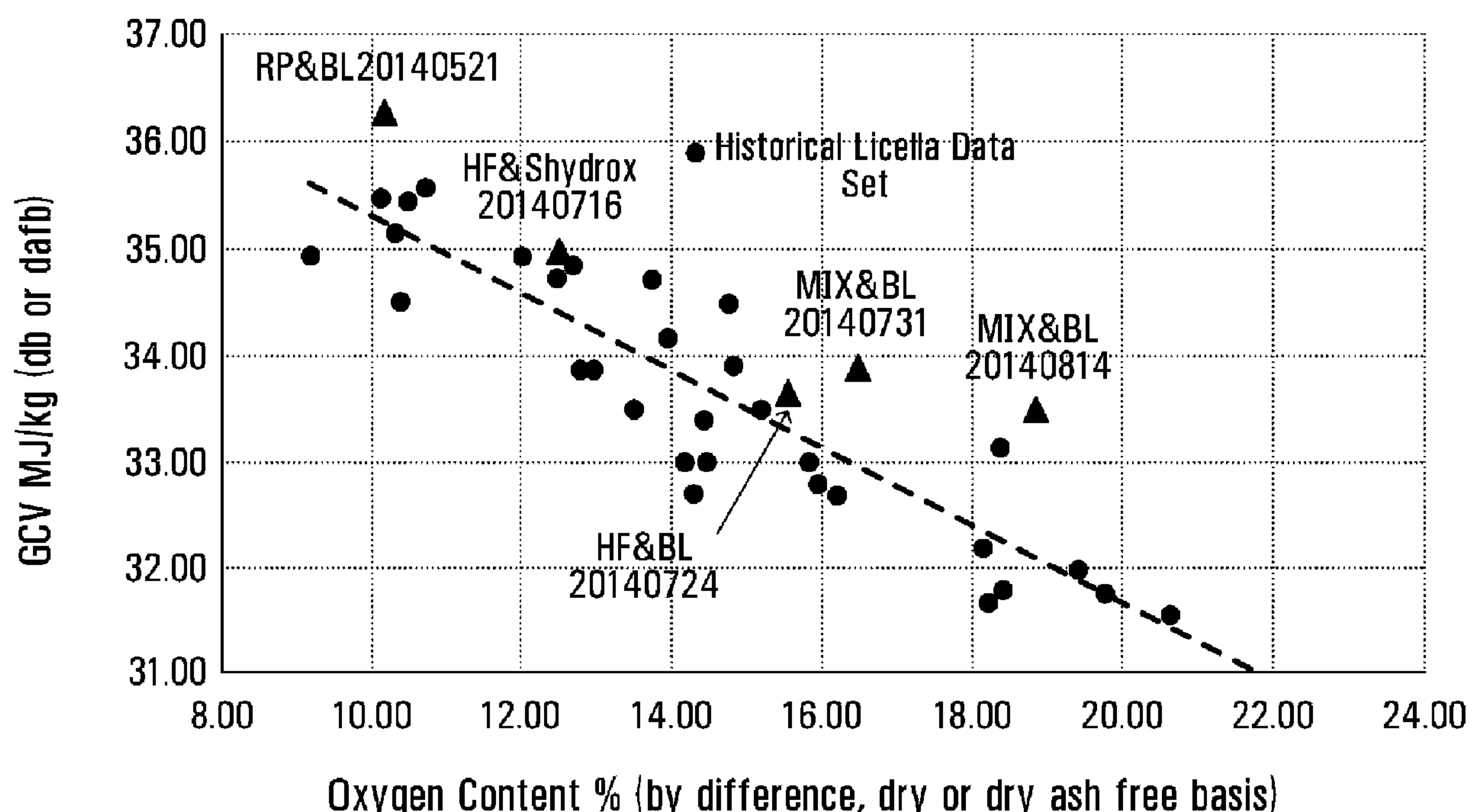
FIG. 1 Biocrude - Gross Calorific Value vs Oxygen Content
