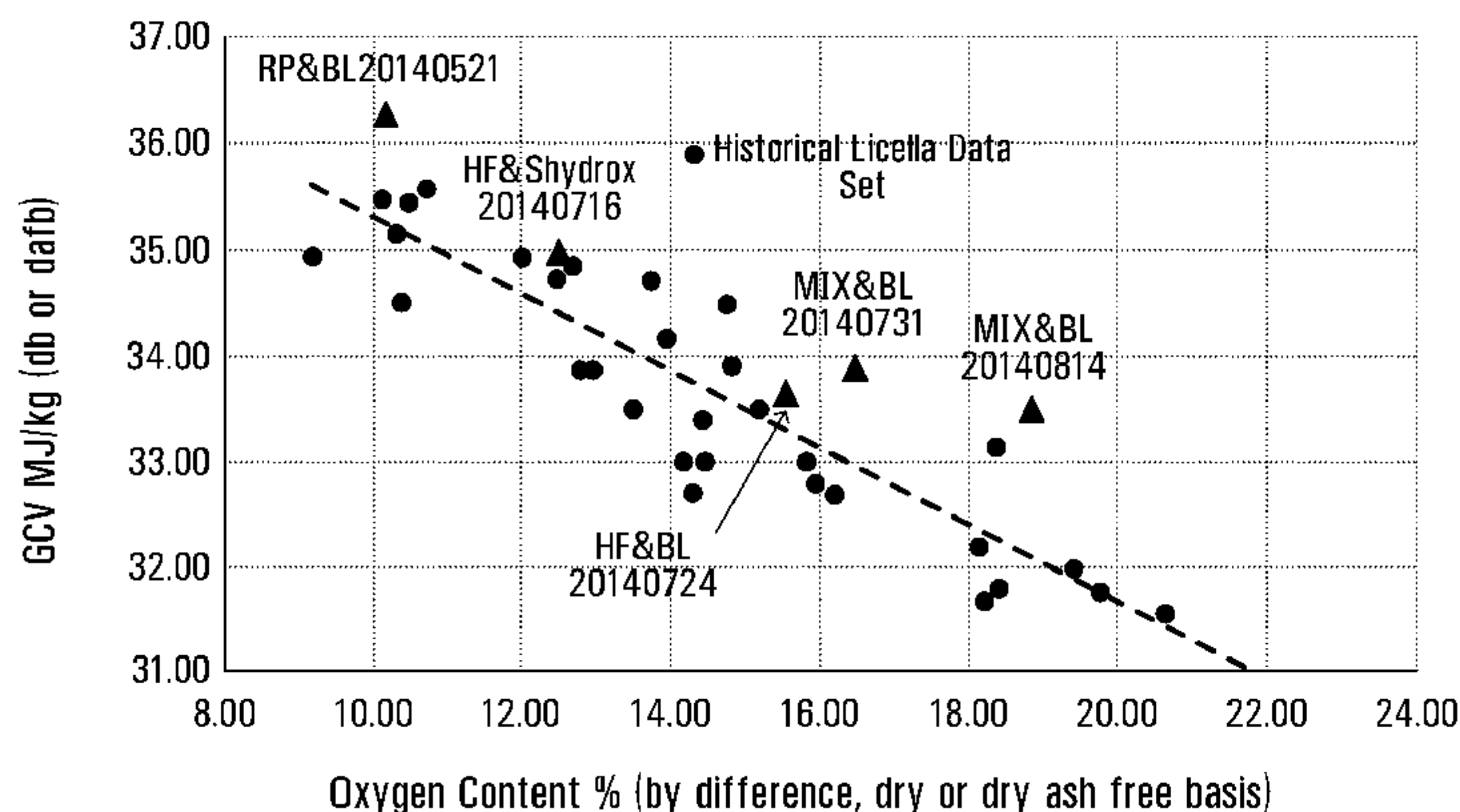
FIG. 1 Biocrude - Gross Calorific Value vs Oxygen Content
