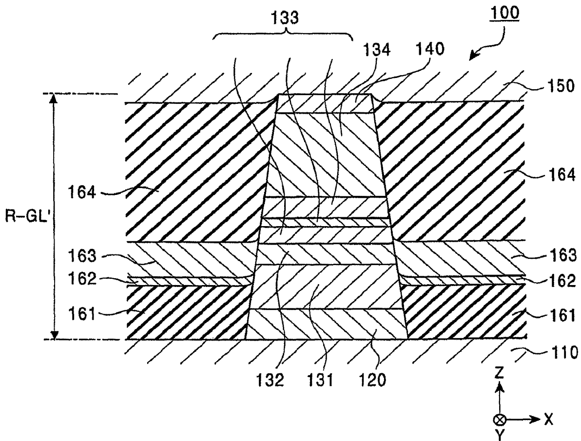
FIG. 21 PRIOR ART
