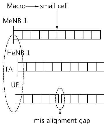
(a) Gap due to mis alignment
