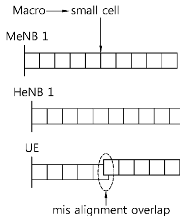
(b) overlap due to mis alignment
