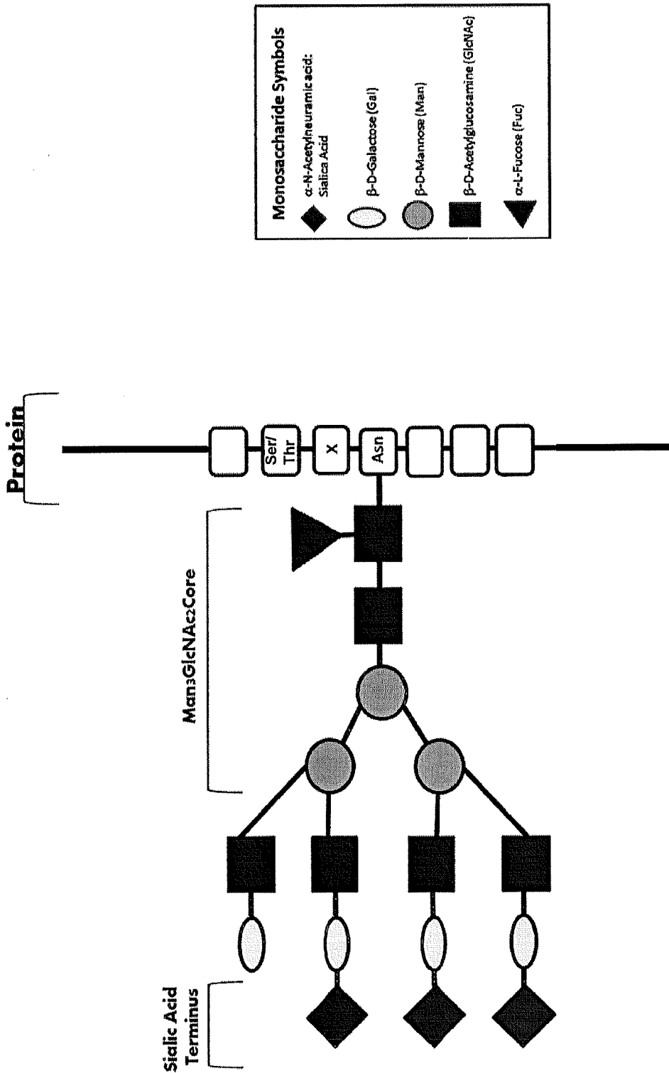
Example of a complex N-linked glycan Figure 4
