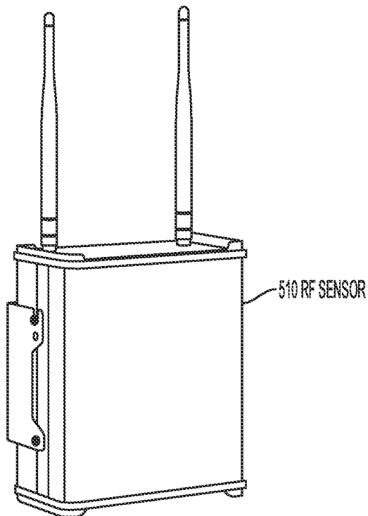
FIG. 5B: EXEMPLARY RF SENSOR DEVICE
