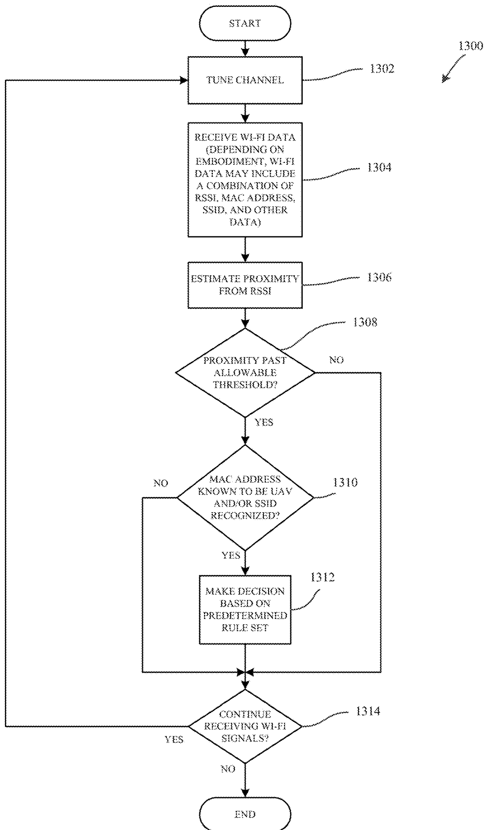
FIG. 13: EXEMPLARY WI-FI DATA ANALYSIS PROCESS
