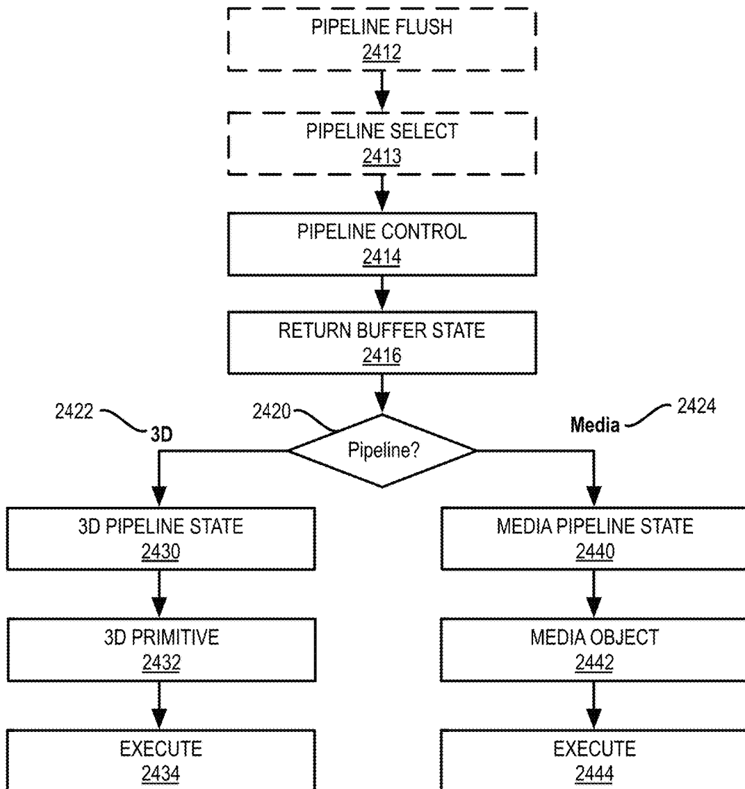
GRAPHICS PROCESSOR COMMAND SEQUENCE
