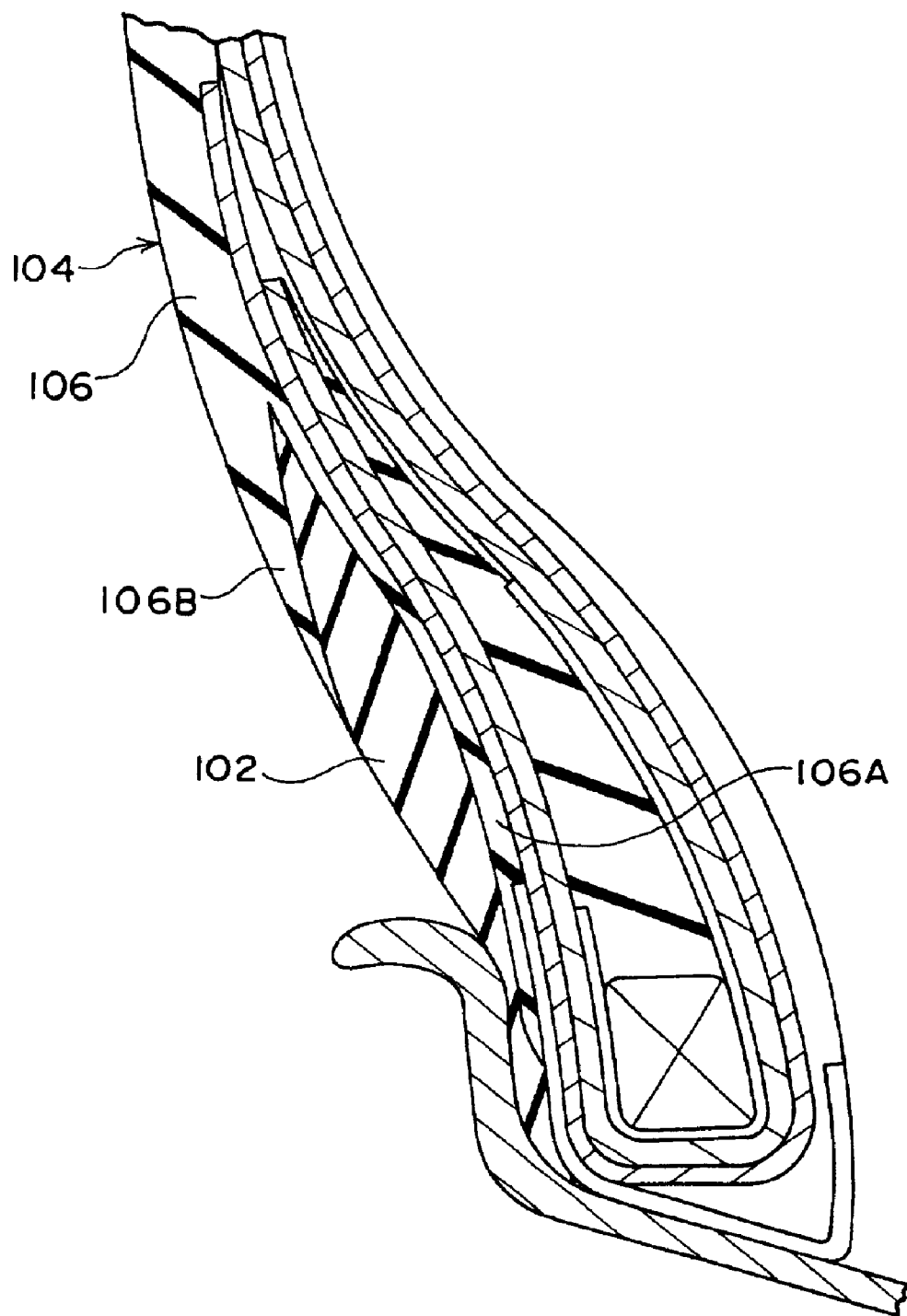
FIG. 7 PRIOR ART
