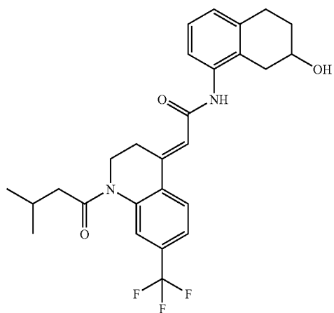
EXAMPLE 87
