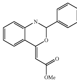
Formula (1)3 RN = 685110-67-2
