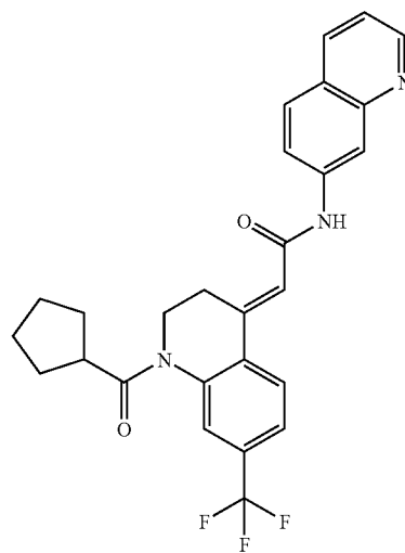
EXAMPLE 70
