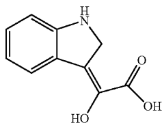
Formula (5) RN = 581874-6
