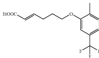
EXAMPLE 6-4
