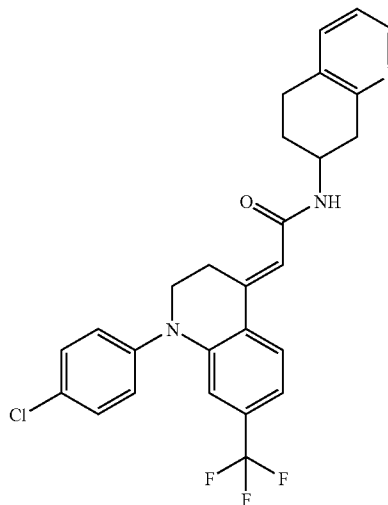
EXAMPLE 54
