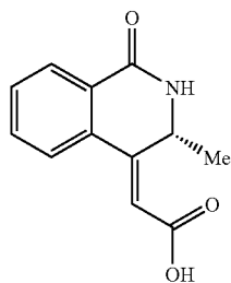
Formula (8) RN = 496802-73-4
