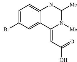
Formula (1)4 RN = 221198-87-4
