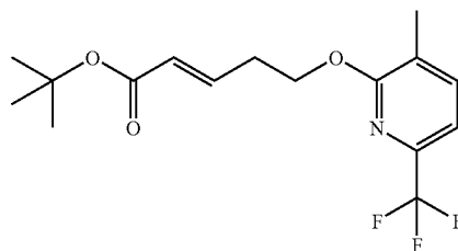
EXAMPLE 235-8
