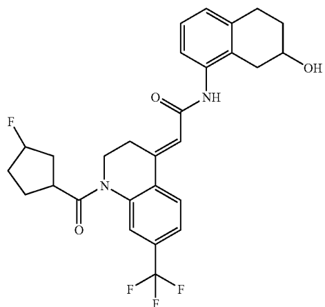
EXAMPLE 88
