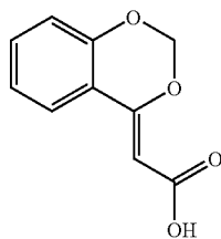
Formula (6) RN = 4442-50-6
