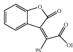
Formula (2) RN = 374919-95-6
