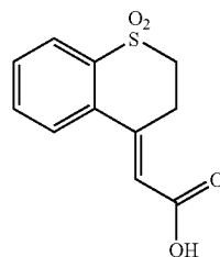
Formula (1)1 RN = 134997-72-1
