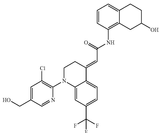
EXAMPLE 200
