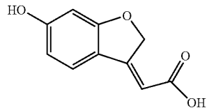
Formula (1)2 RN = 855221-04-4
