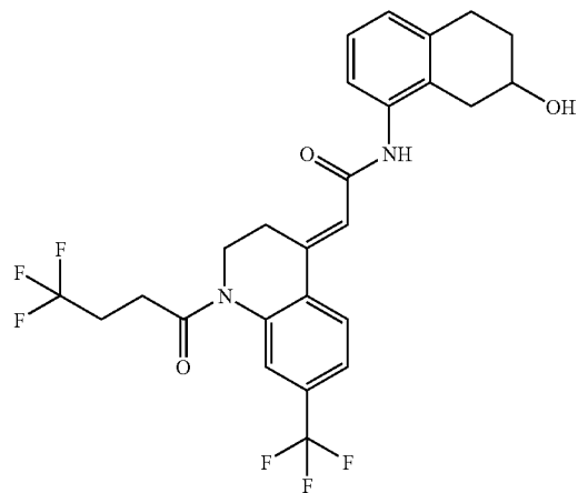
EXAMPLE 91
