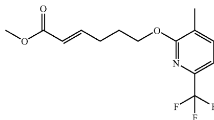
EXAMPLE 237-2
