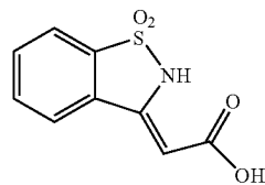
Formula (10) RN = 34981-46-9
