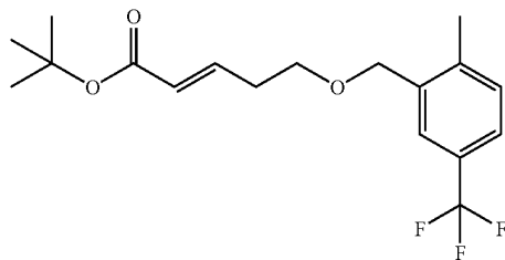
EXAMPLE 235-10
