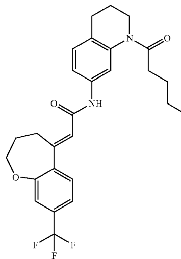
EXAMPLE 150
