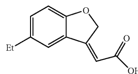
Formula (1) RN = 879935-05-5
