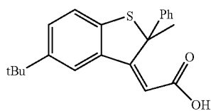
Formula (7) RN = 869593-14-6
