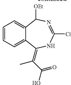
Formula (3) RN = 300695-65-2
