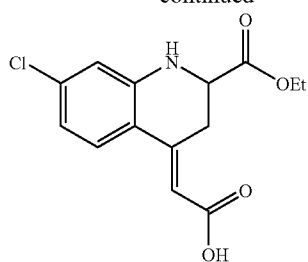
Formula (9) RN = 294626-49-6
