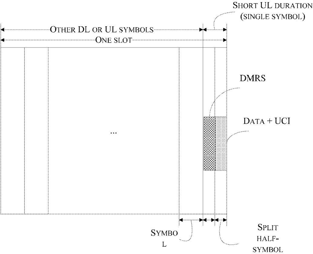
Figure 1C (Prior Art)
